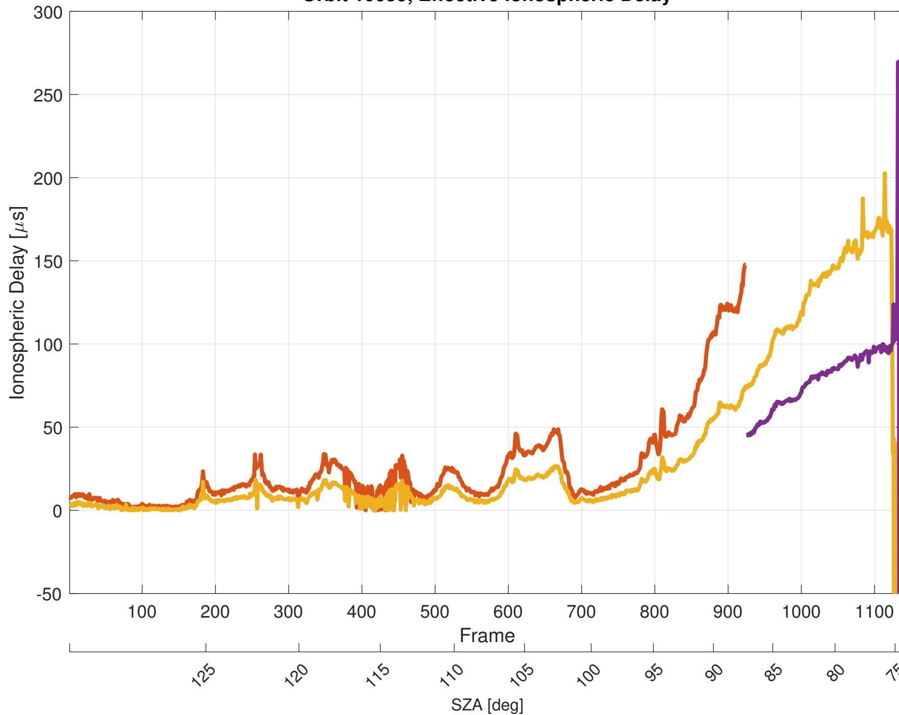
Orbit 10059, Effective Ionospheric Delay
