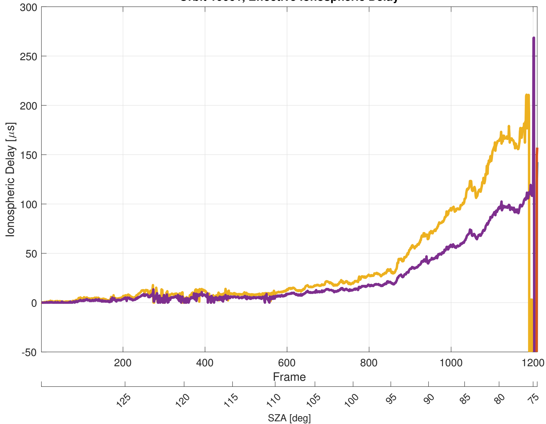
Orbit 10061, Effective Ionospheric Delay
