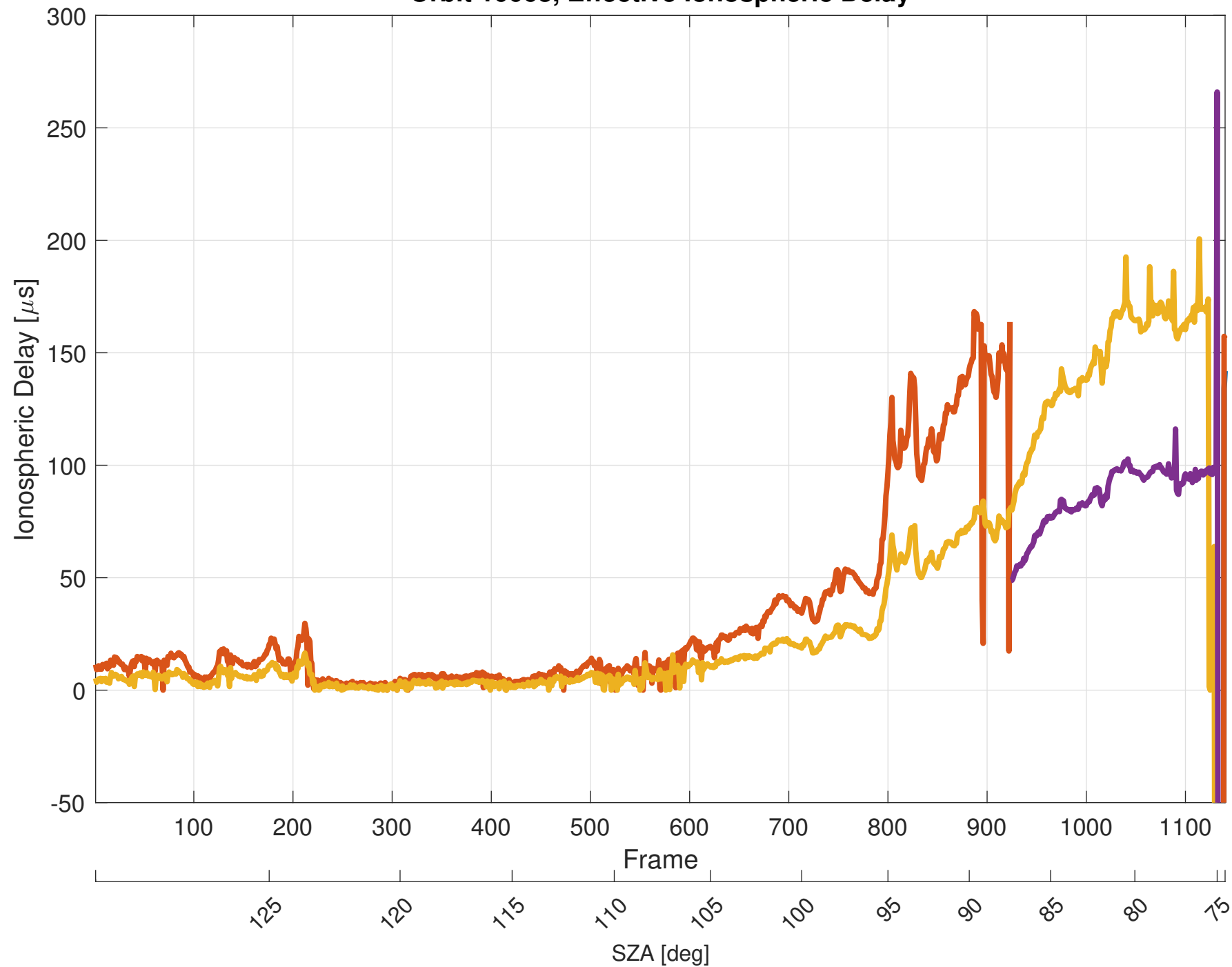
Orbit 10063, Effective Ionospheric Delay
