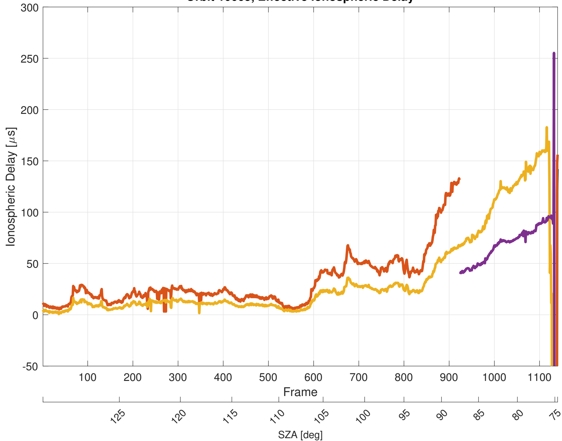
Orbit 10065, Effective Ionospheric Delay
