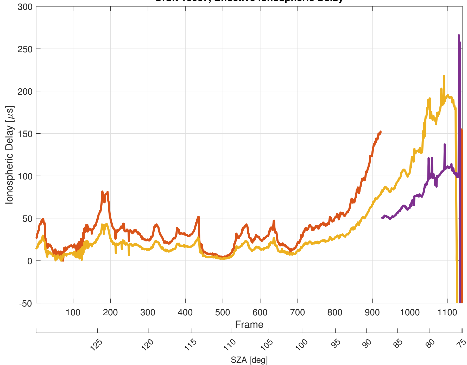
Orbit 10067, Effective Ionospheric Delay
