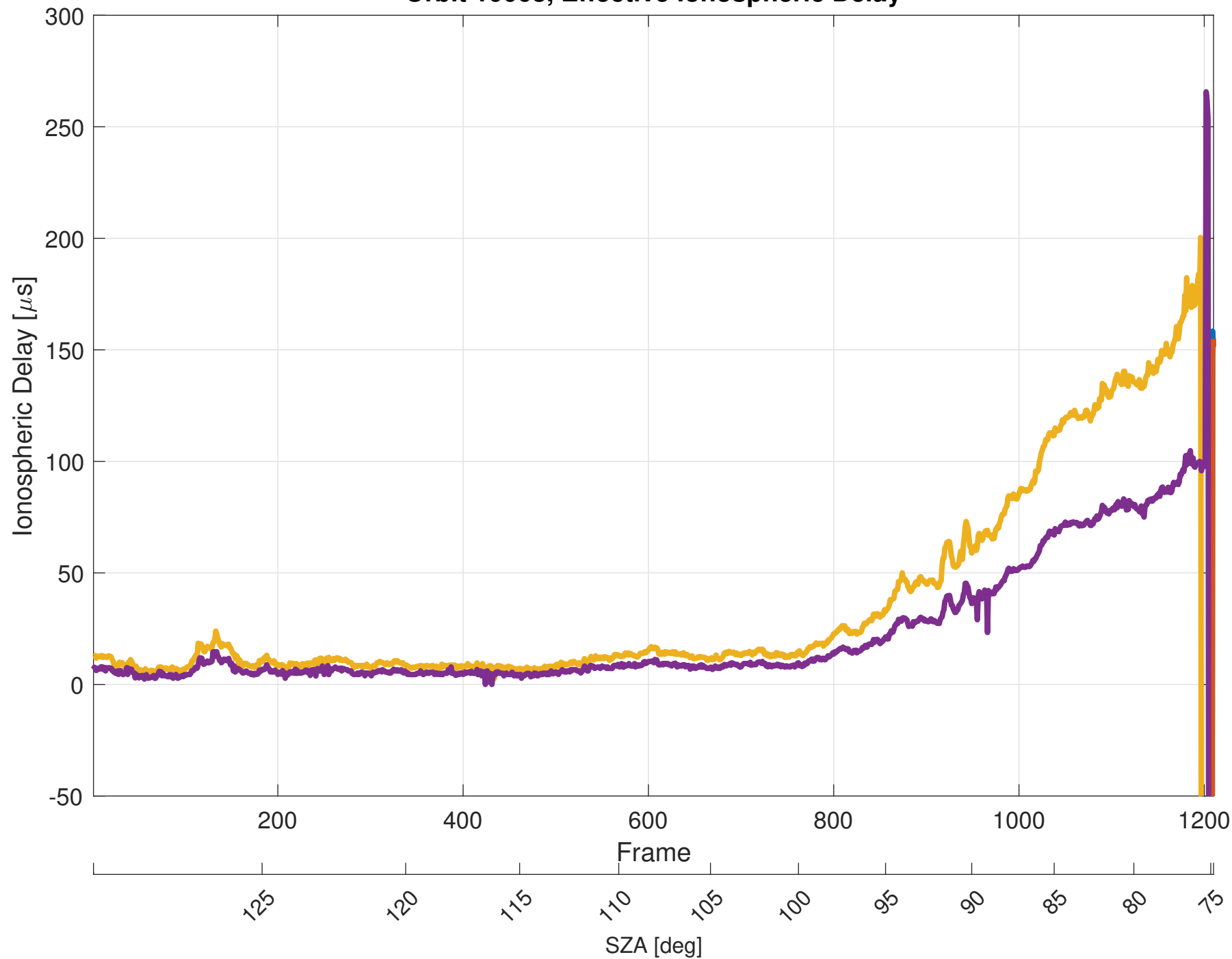
Orbit 10068, Effective Ionospheric Delay
