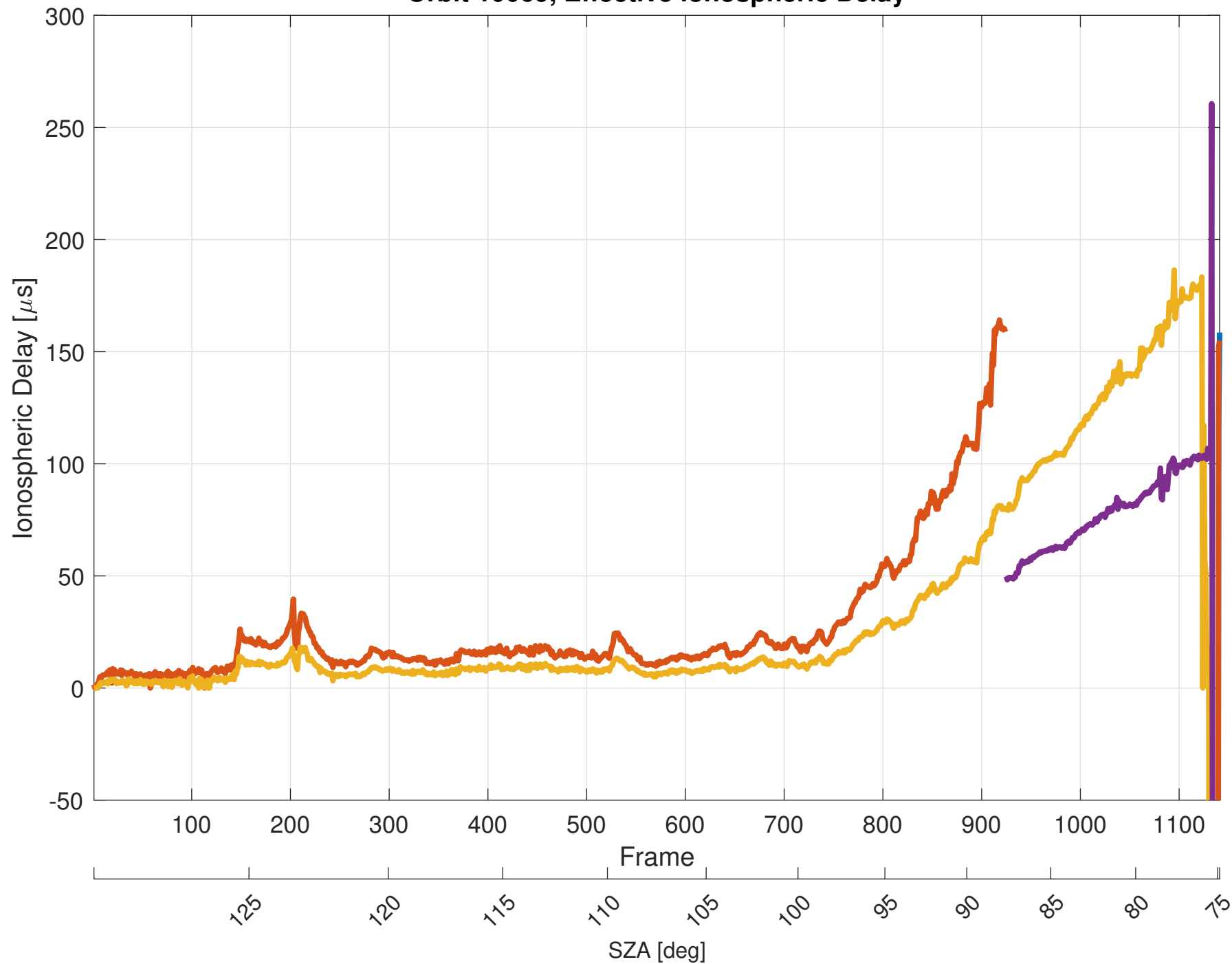
Orbit 10069, Effective Ionospheric Delay
