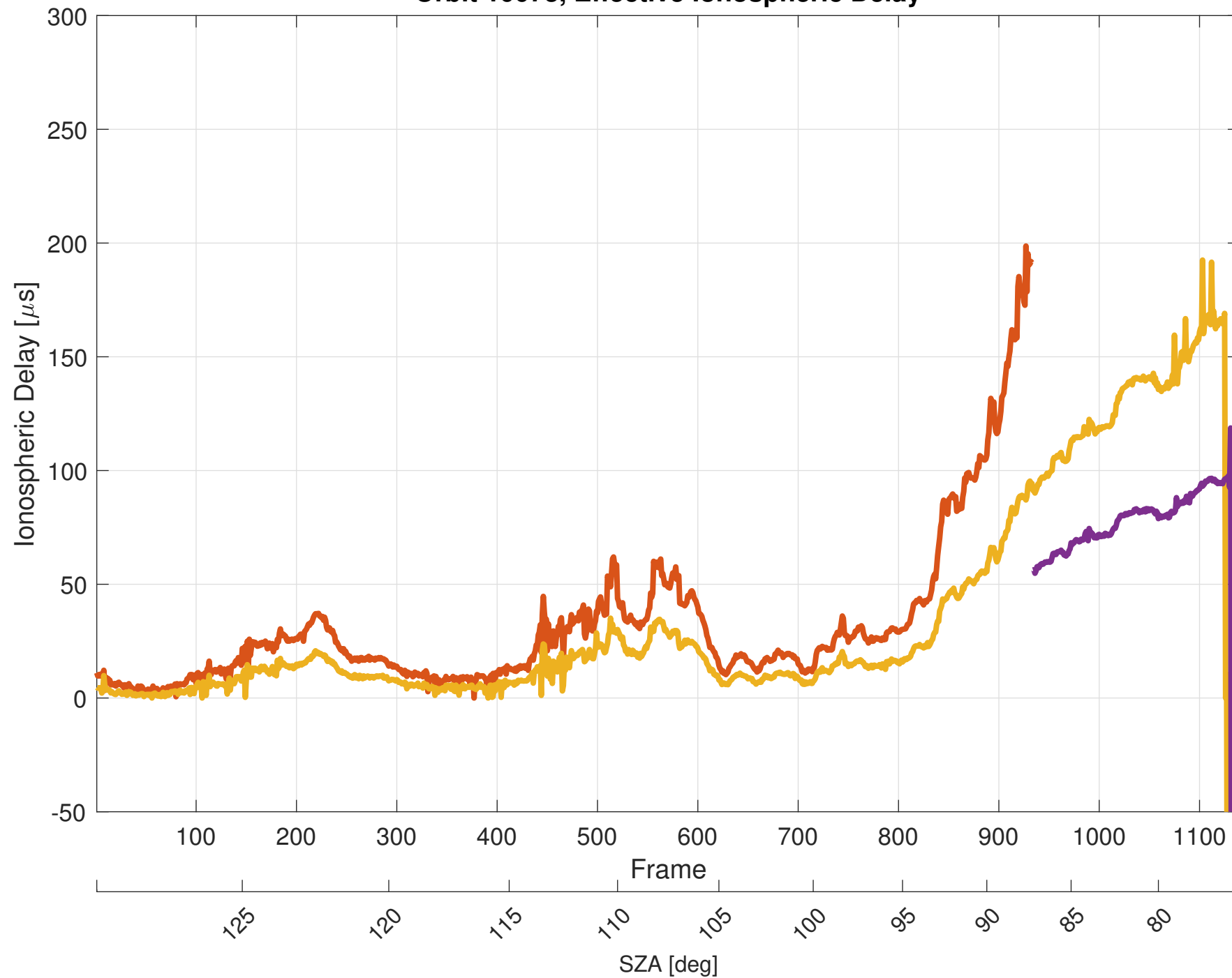
Orbit 10073, Effective Ionospheric Delay
