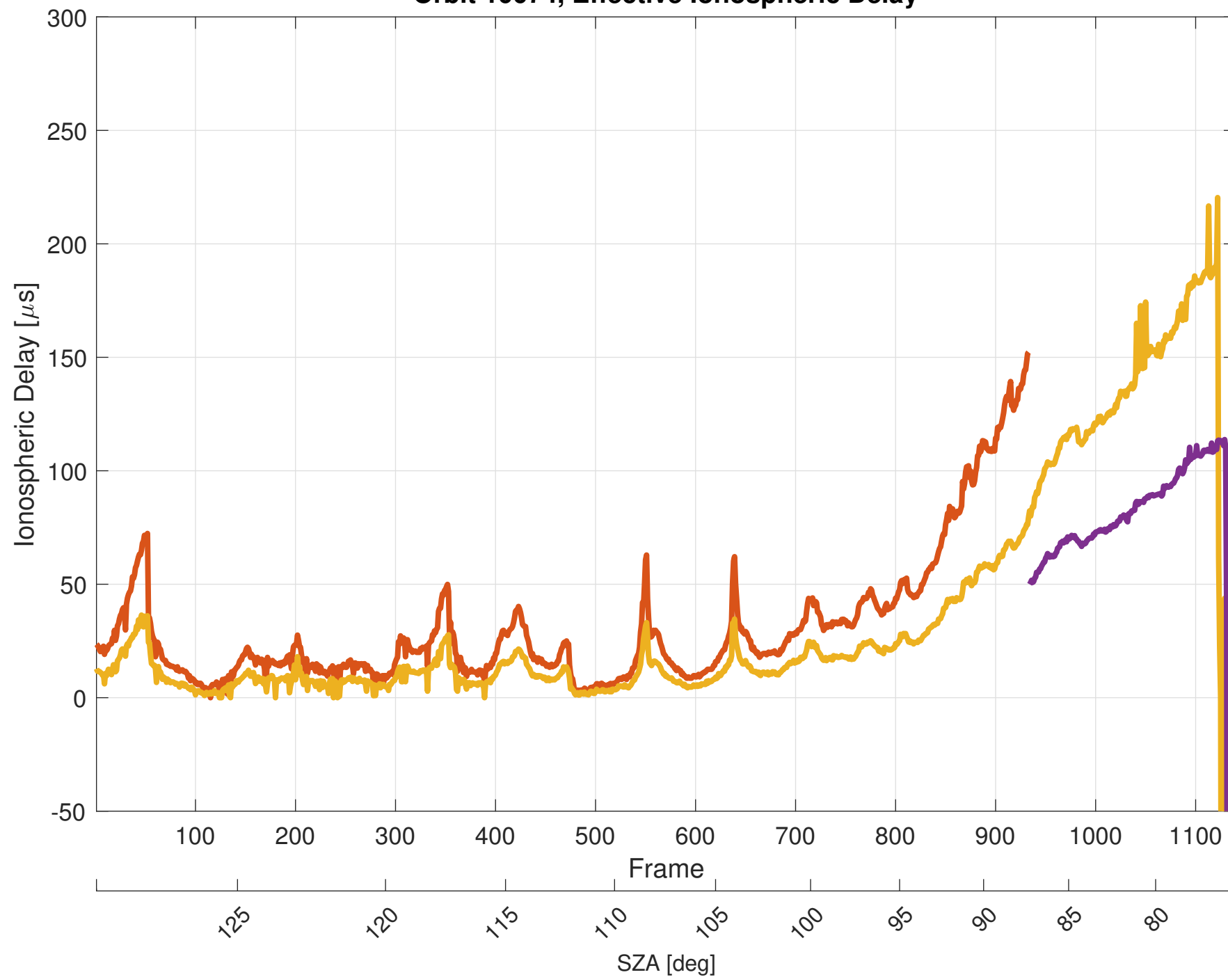
Orbit 10074, Effective Ionospheric Delay
