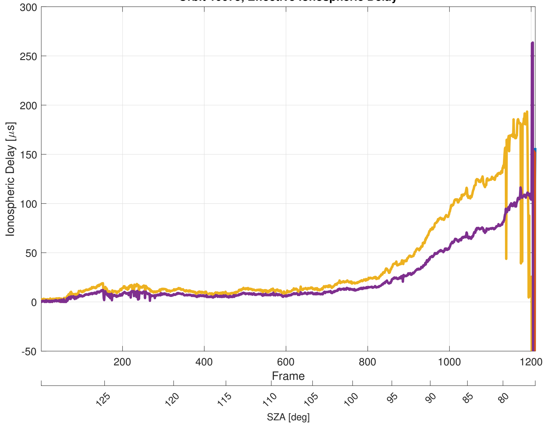
Orbit 10075, Effective Ionospheric Delay
