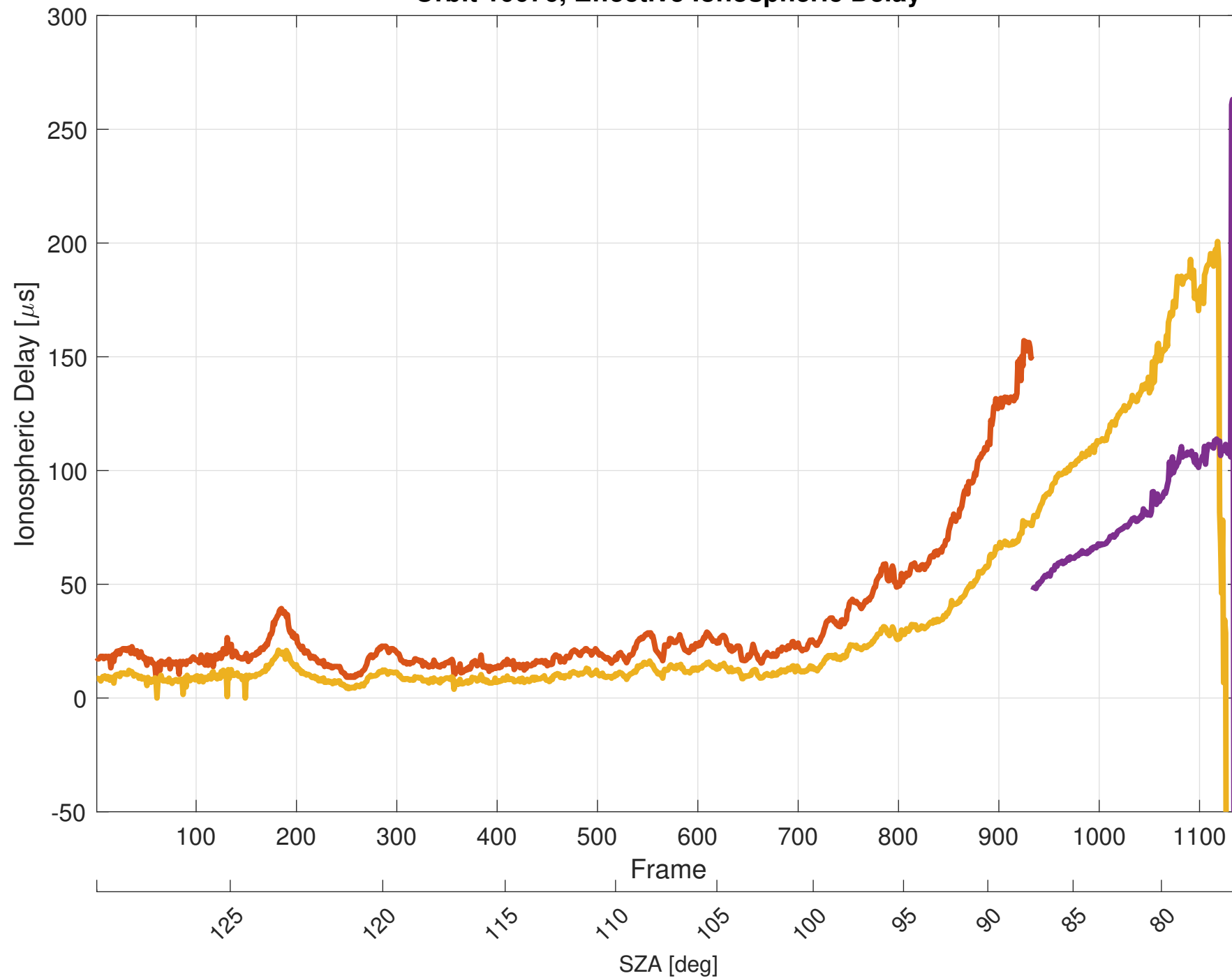
Orbit 10076, Effective Ionospheric Delay
