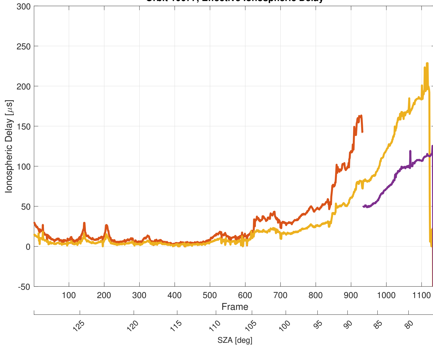
Orbit 10077, Effective Ionospheric Delay
