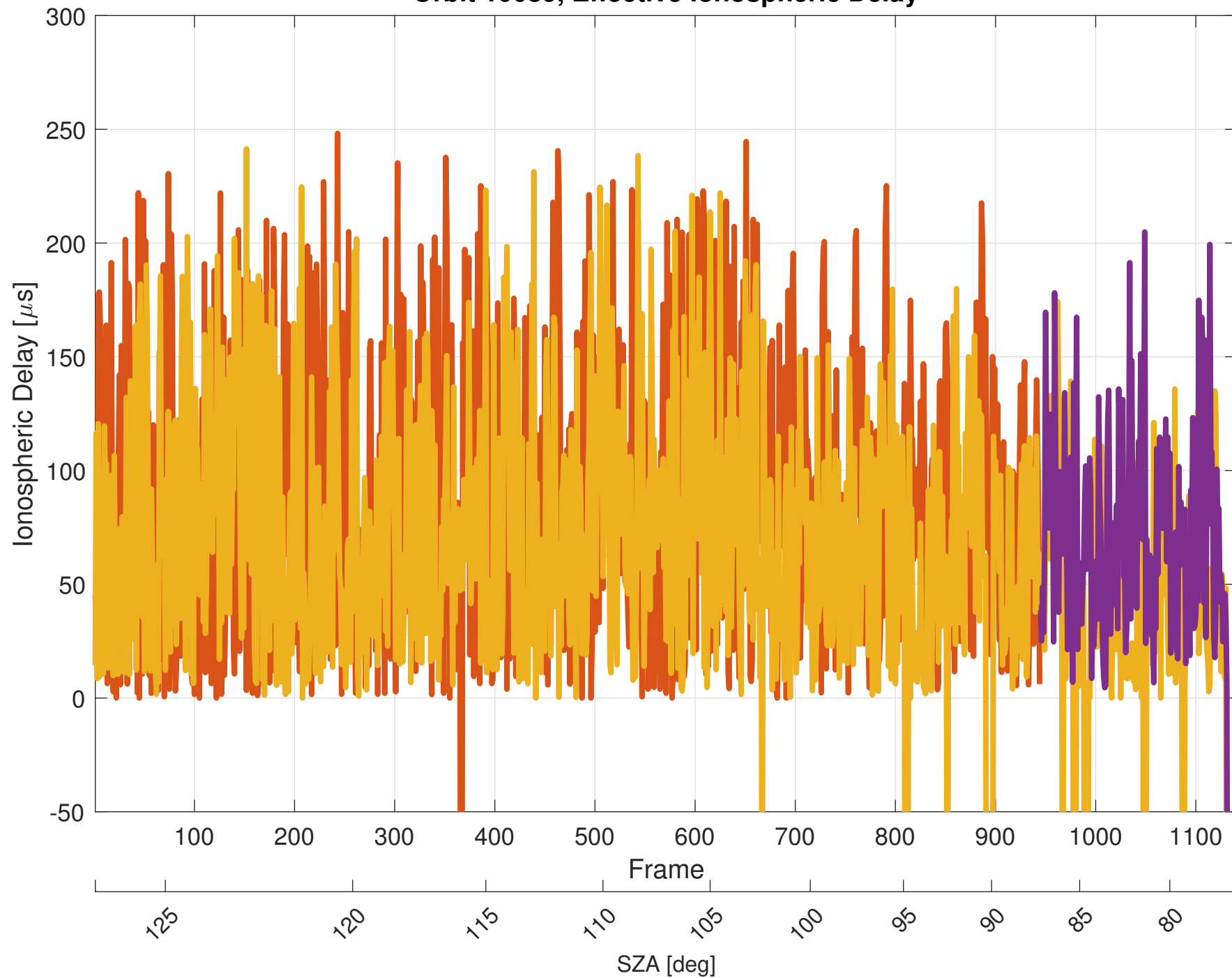
Orbit 10089, Effective Ionospheric Delay
