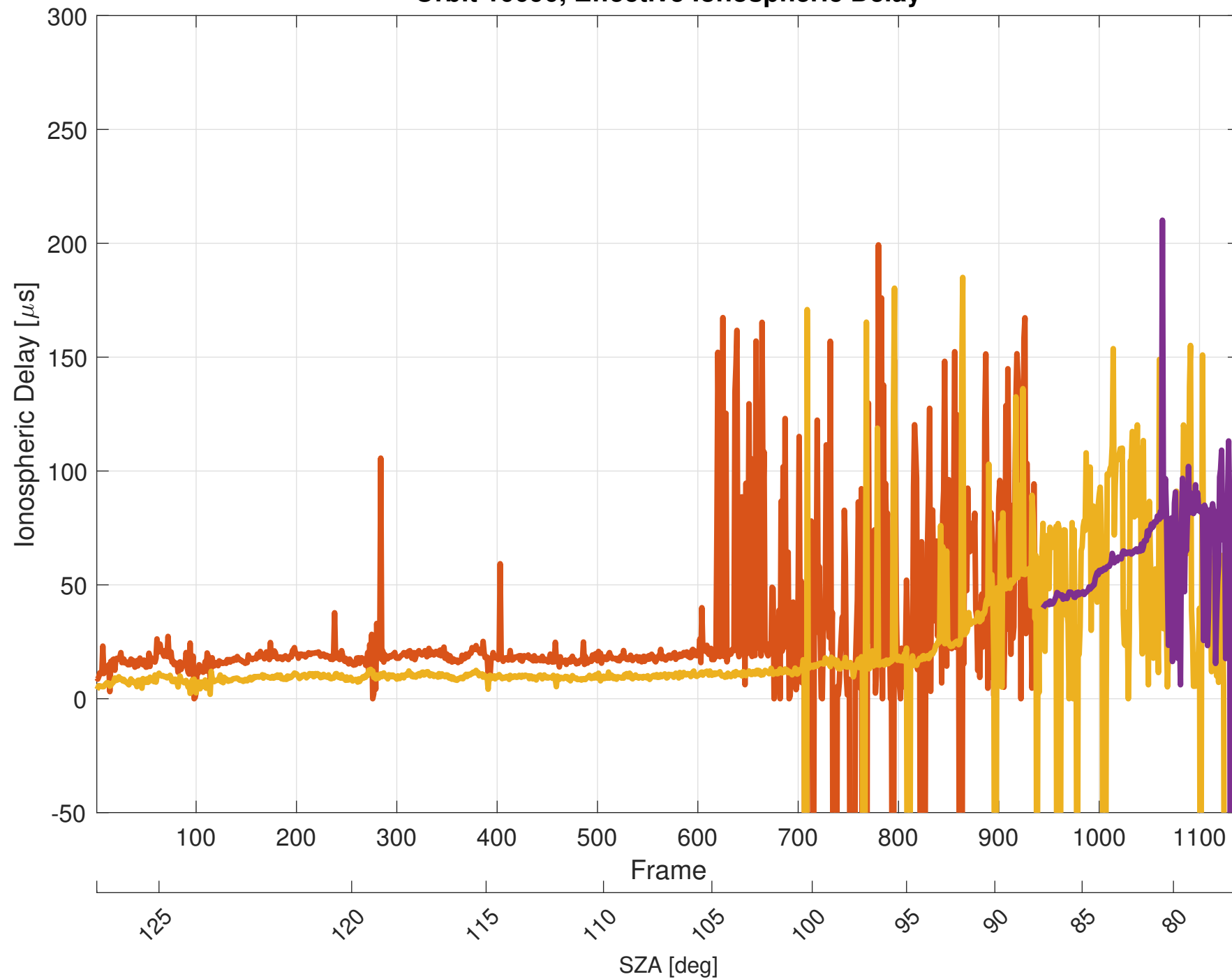
Orbit 10090, Effective Ionospheric Delay
