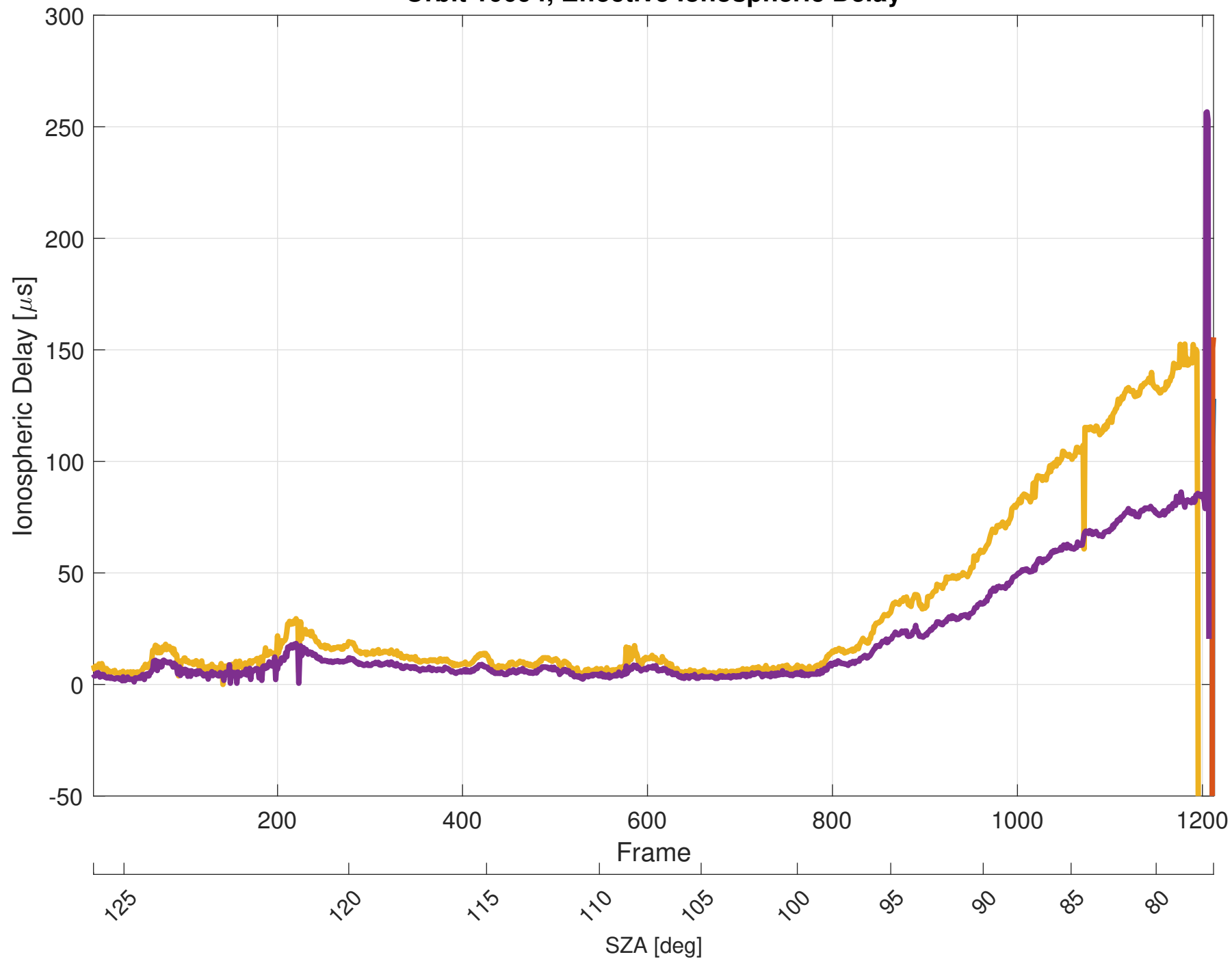
Orbit 10094, Effective Ionospheric Delay
