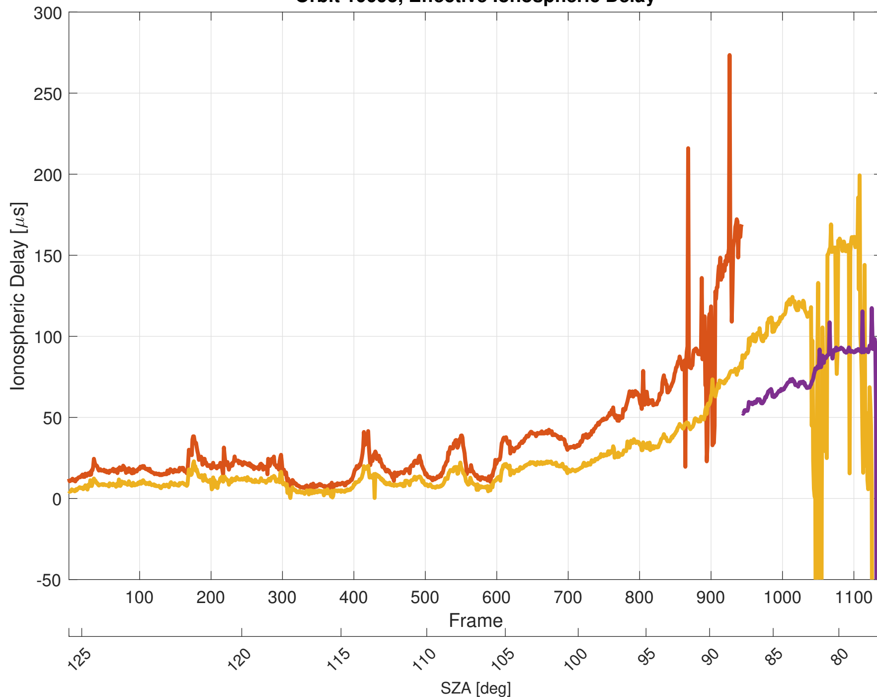
Orbit 10095, Effective Ionospheric Delay
