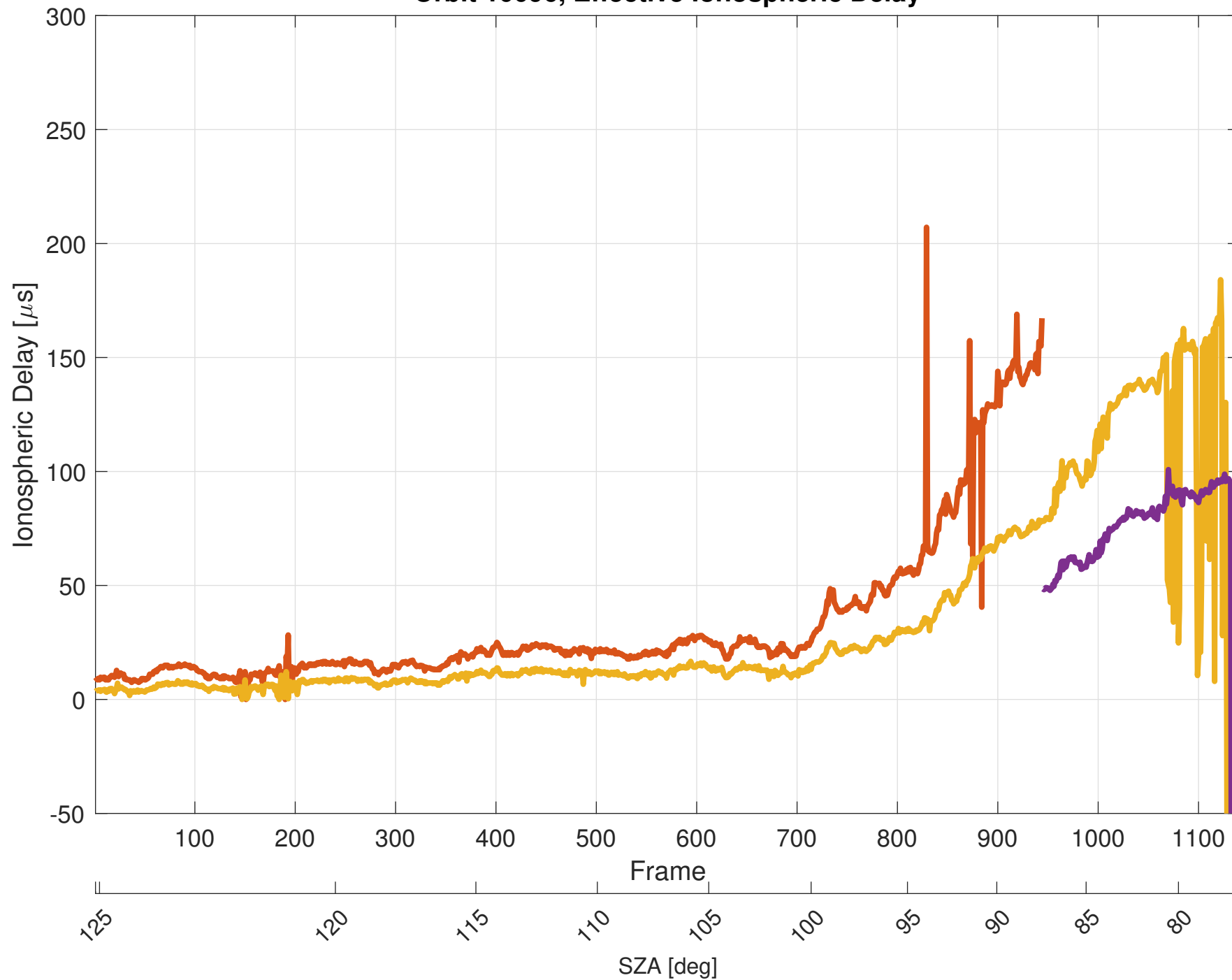
Orbit 10096, Effective Ionospheric Delay
