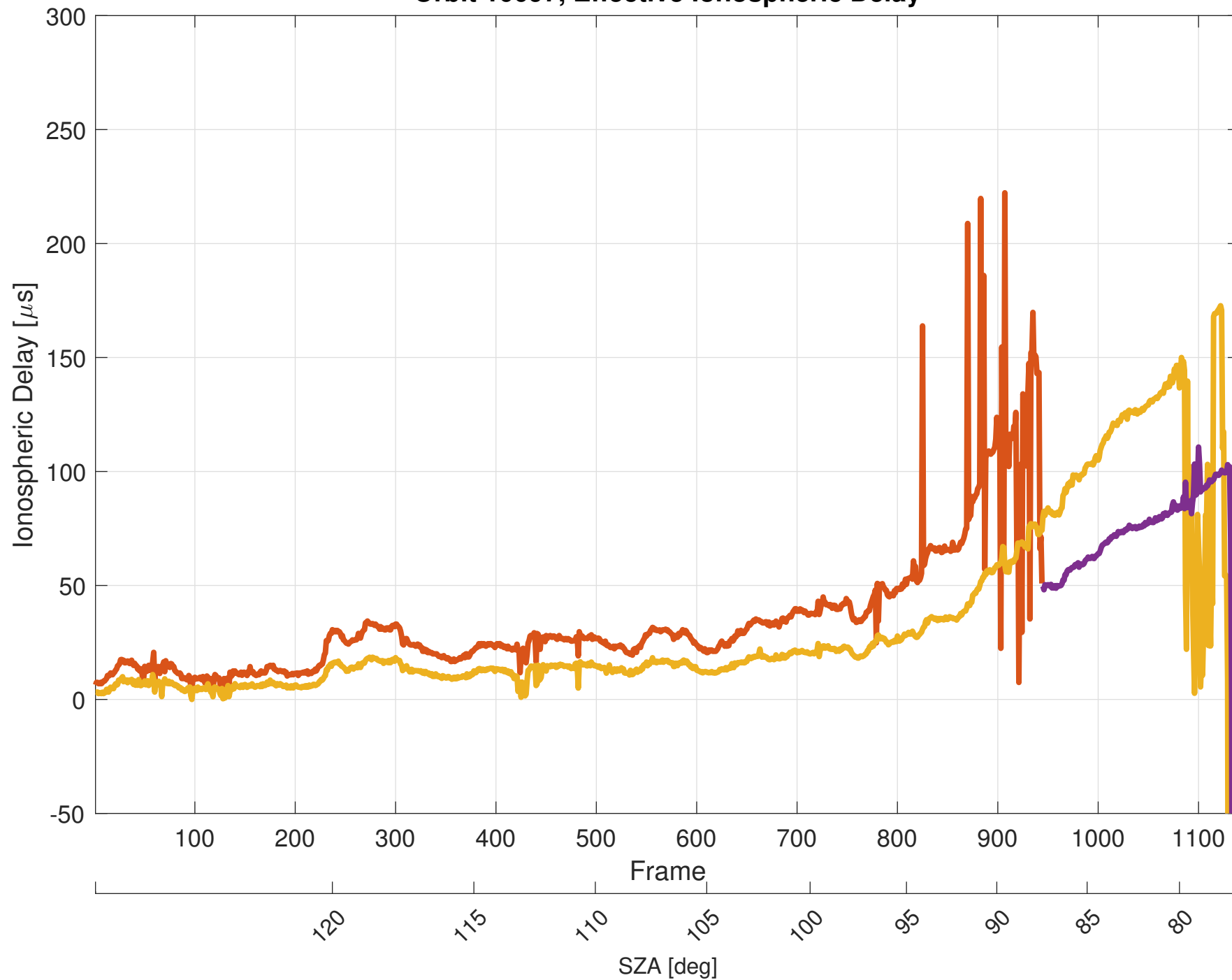
Orbit 10097, Effective Ionospheric Delay
