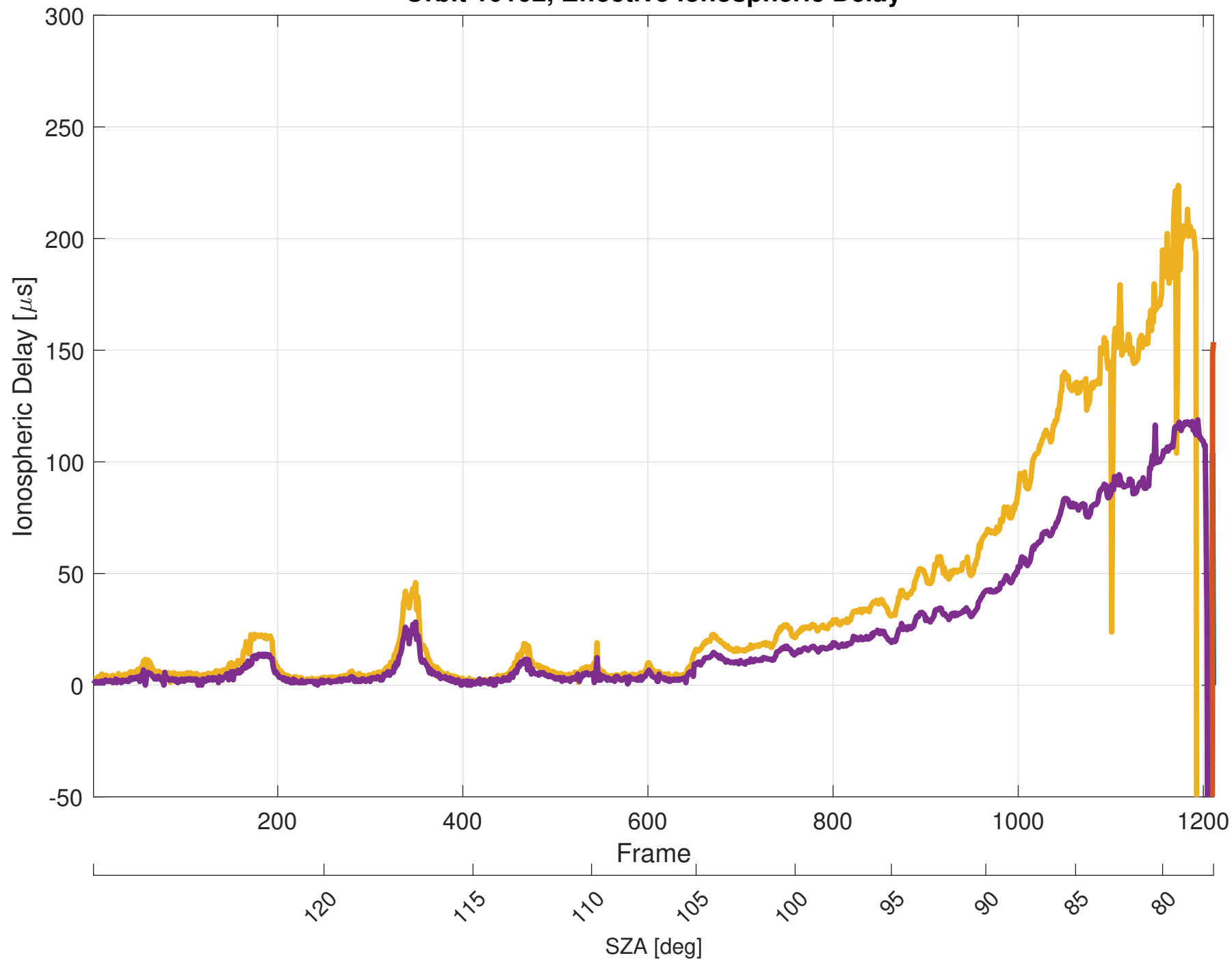
Orbit 10102, Effective Ionospheric Delay
