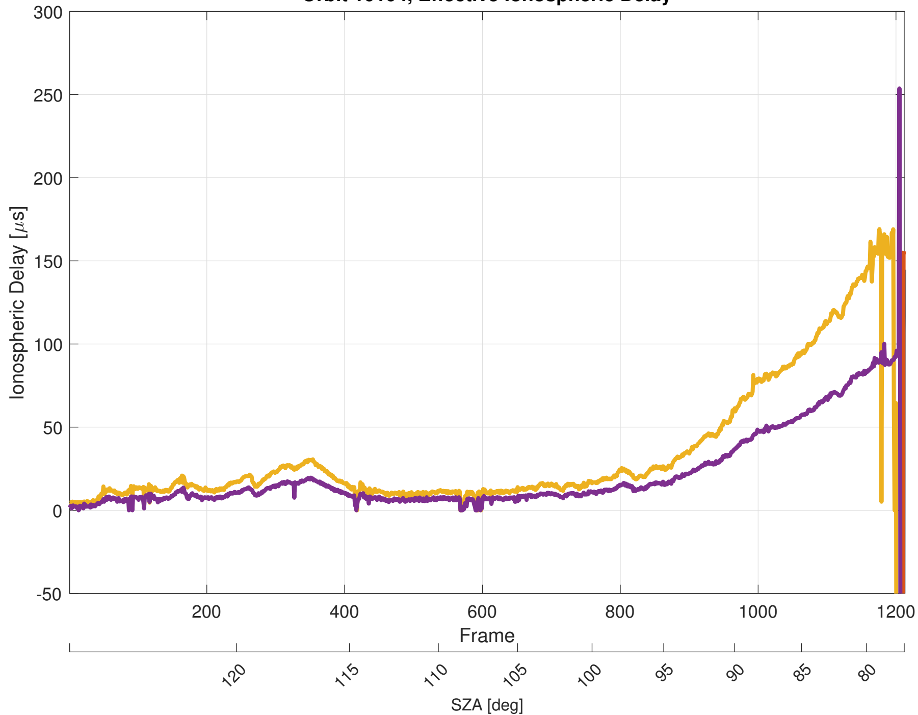
Orbit 10104, Effective Ionospheric Delay
