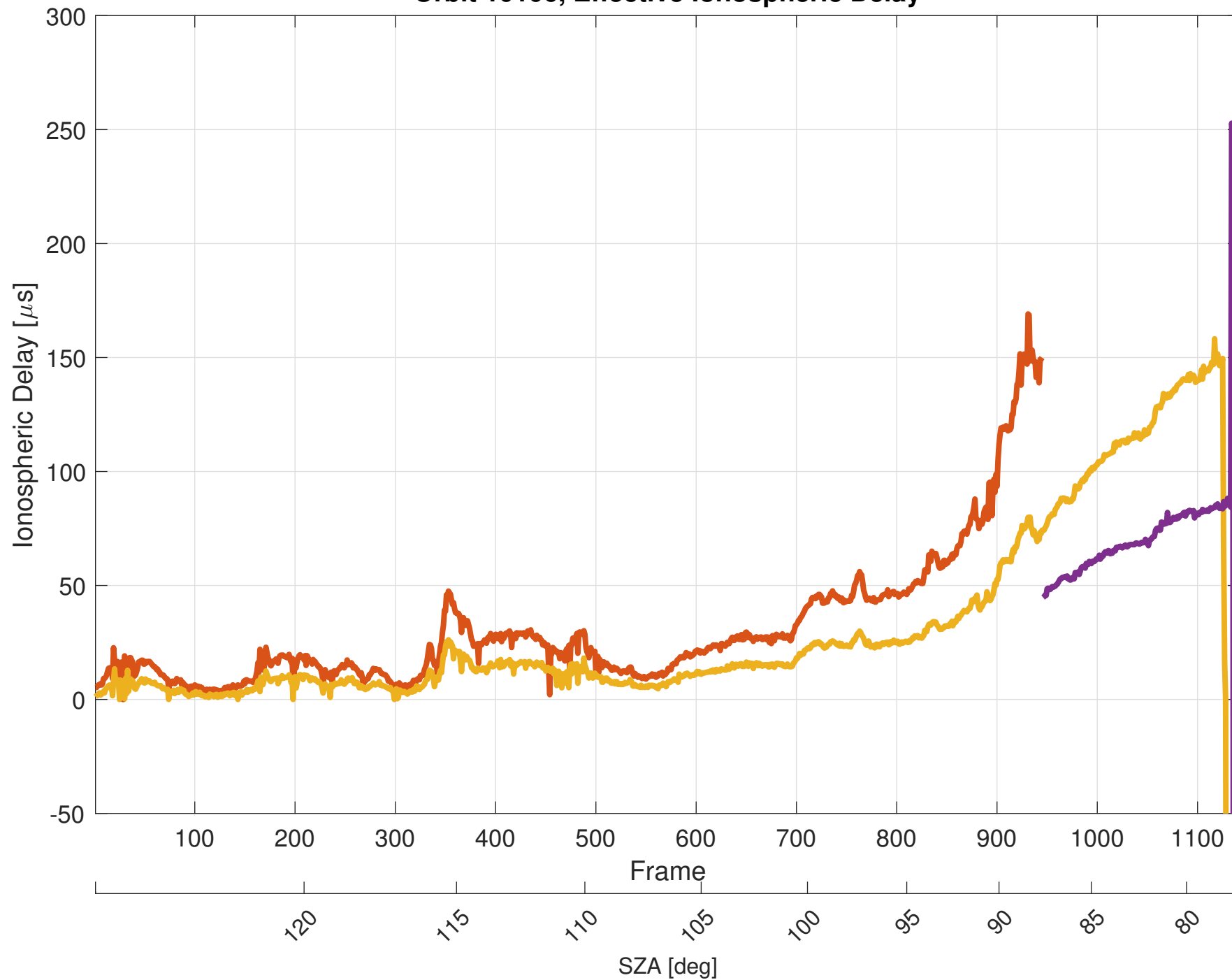
Orbit 10106, Effective Ionospheric Delay
