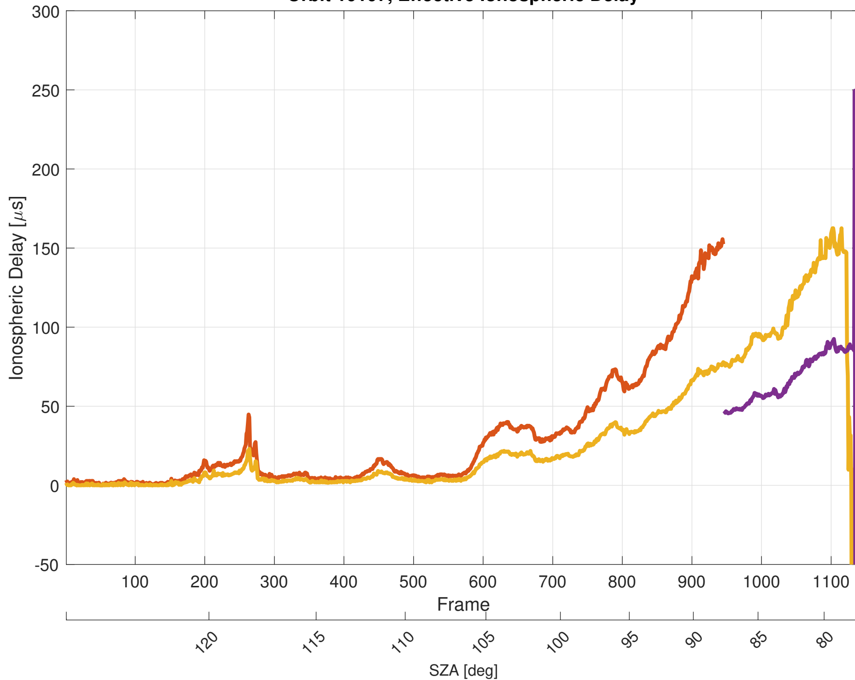
Orbit 10107, Effective Ionospheric Delay
