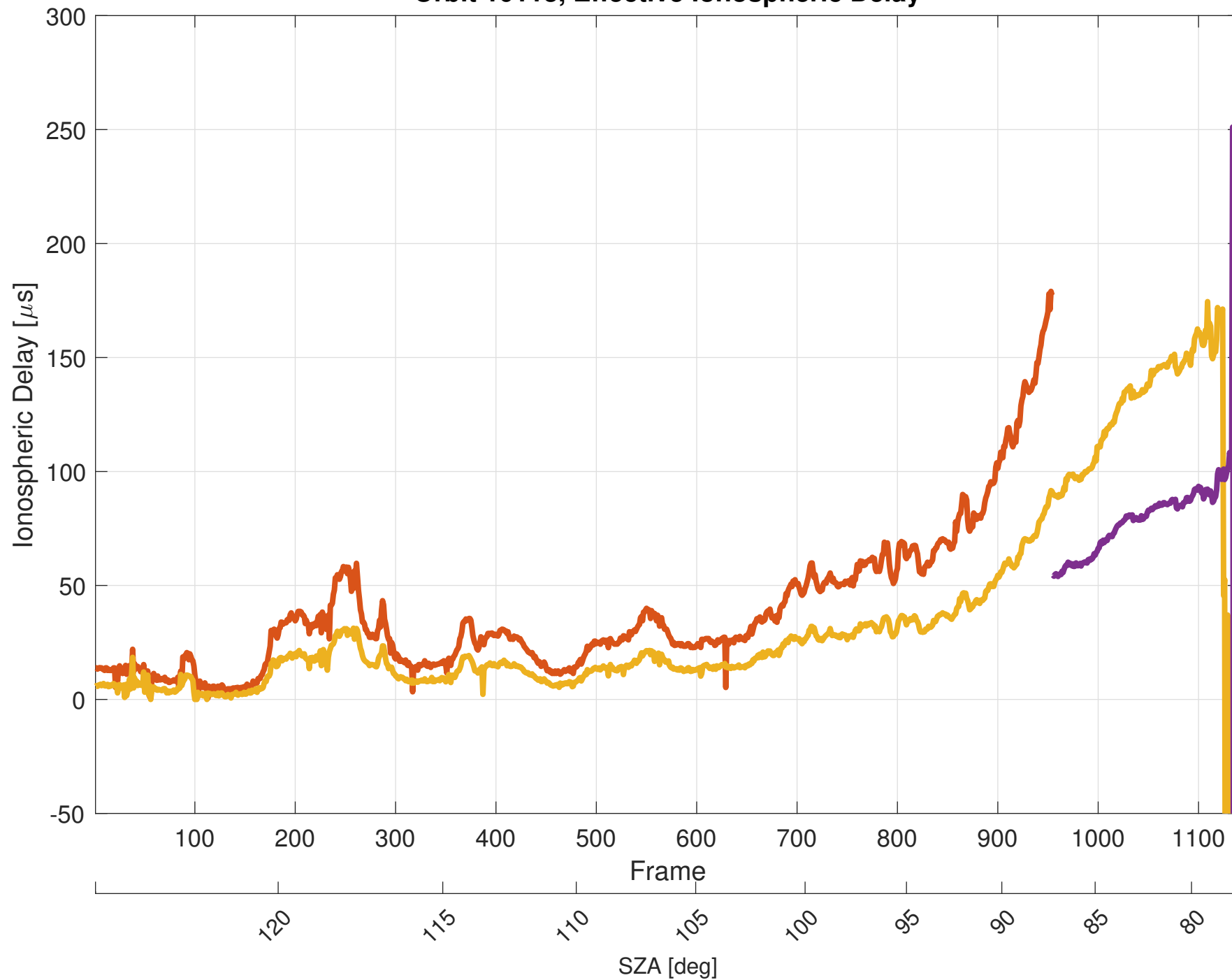
Orbit 10113, Effective Ionospheric Delay
