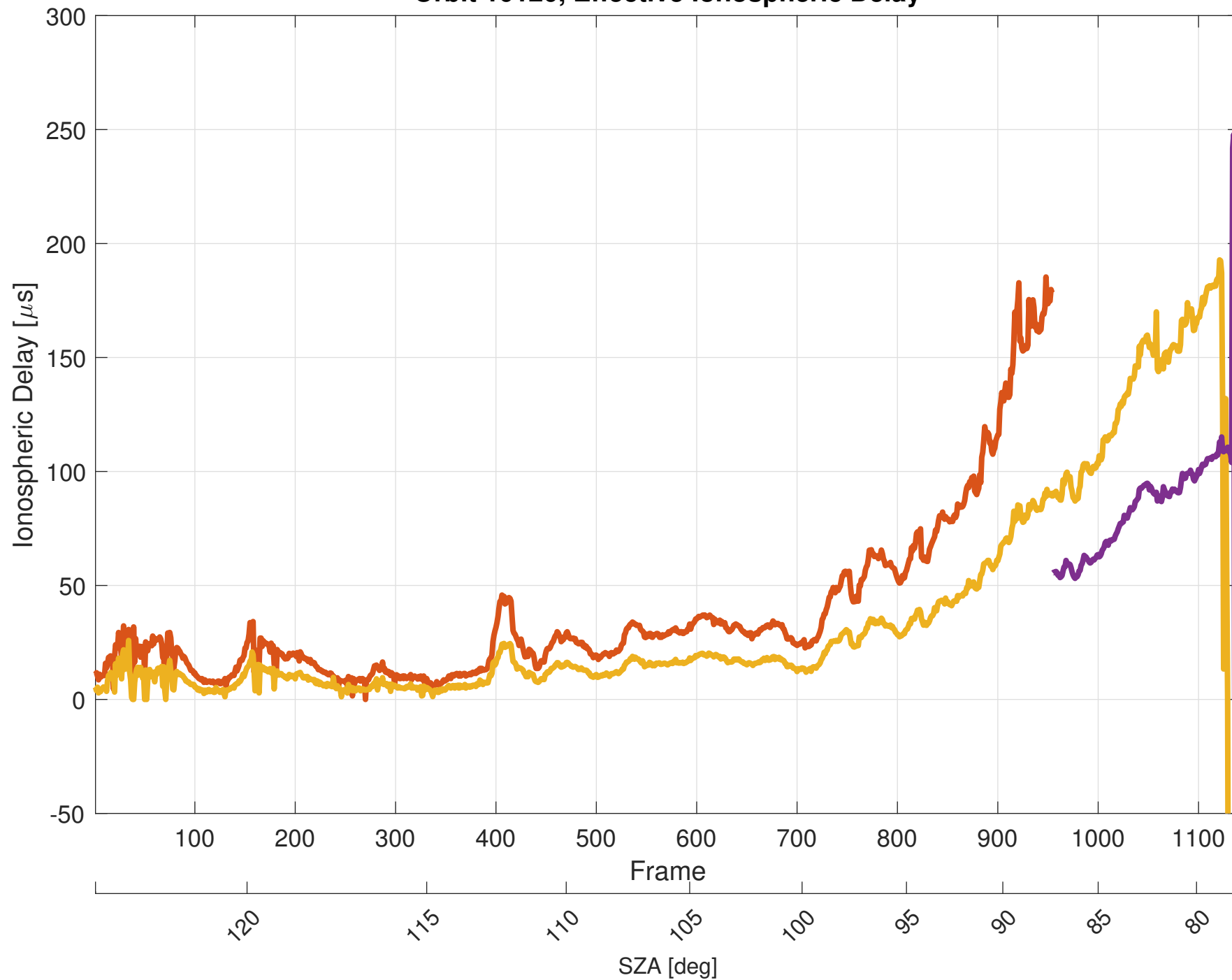
Orbit 10120, Effective Ionospheric Delay
