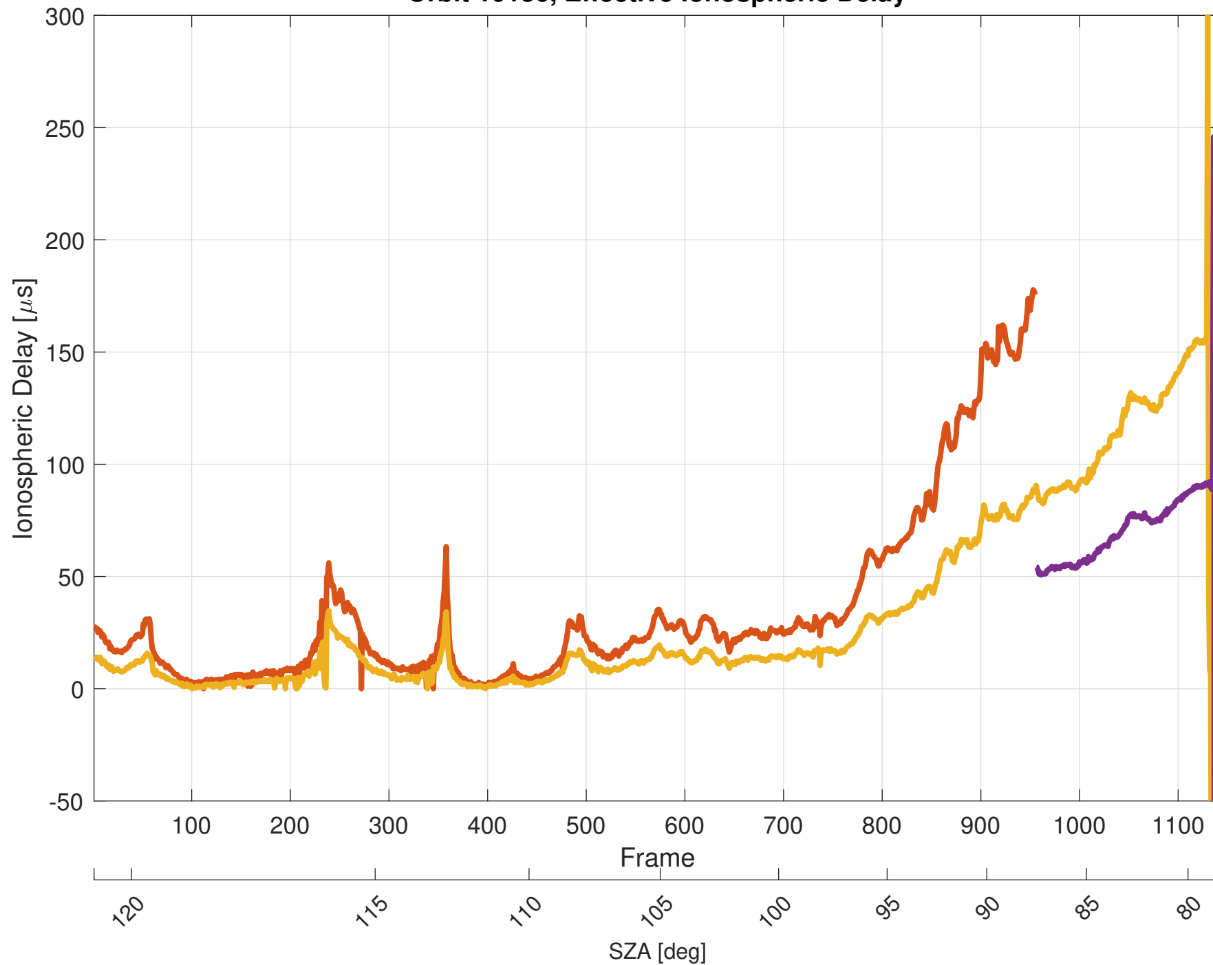
Orbit 10136, Effective Ionospheric Delay
