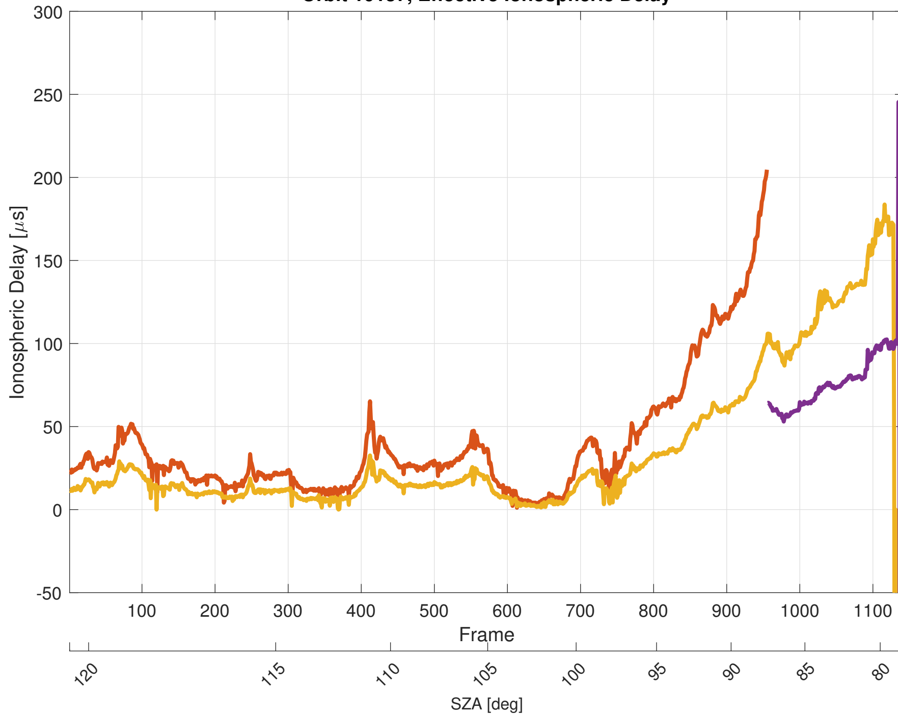
Orbit 10137, Effective Ionospheric Delay
