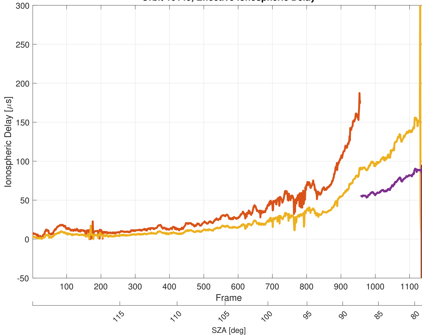
Orbit 10145, Effective Ionospheric Delay
