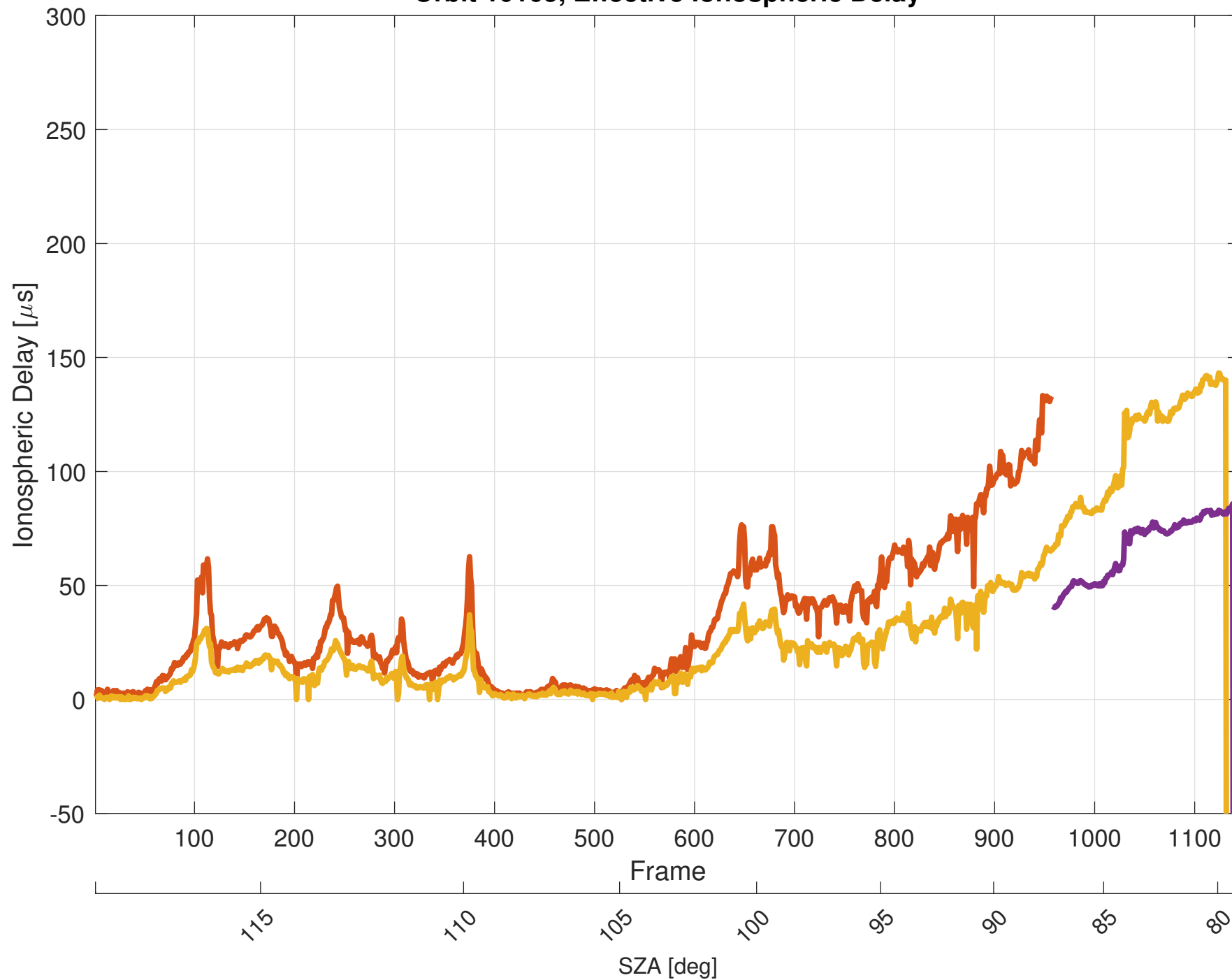
Orbit 10165, Effective Ionospheric Delay
