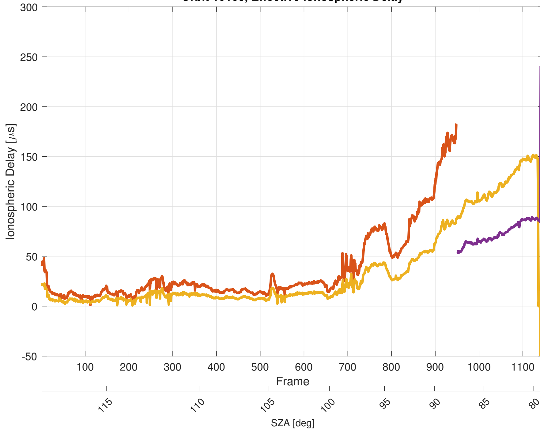
Orbit 10168, Effective Ionospheric Delay
