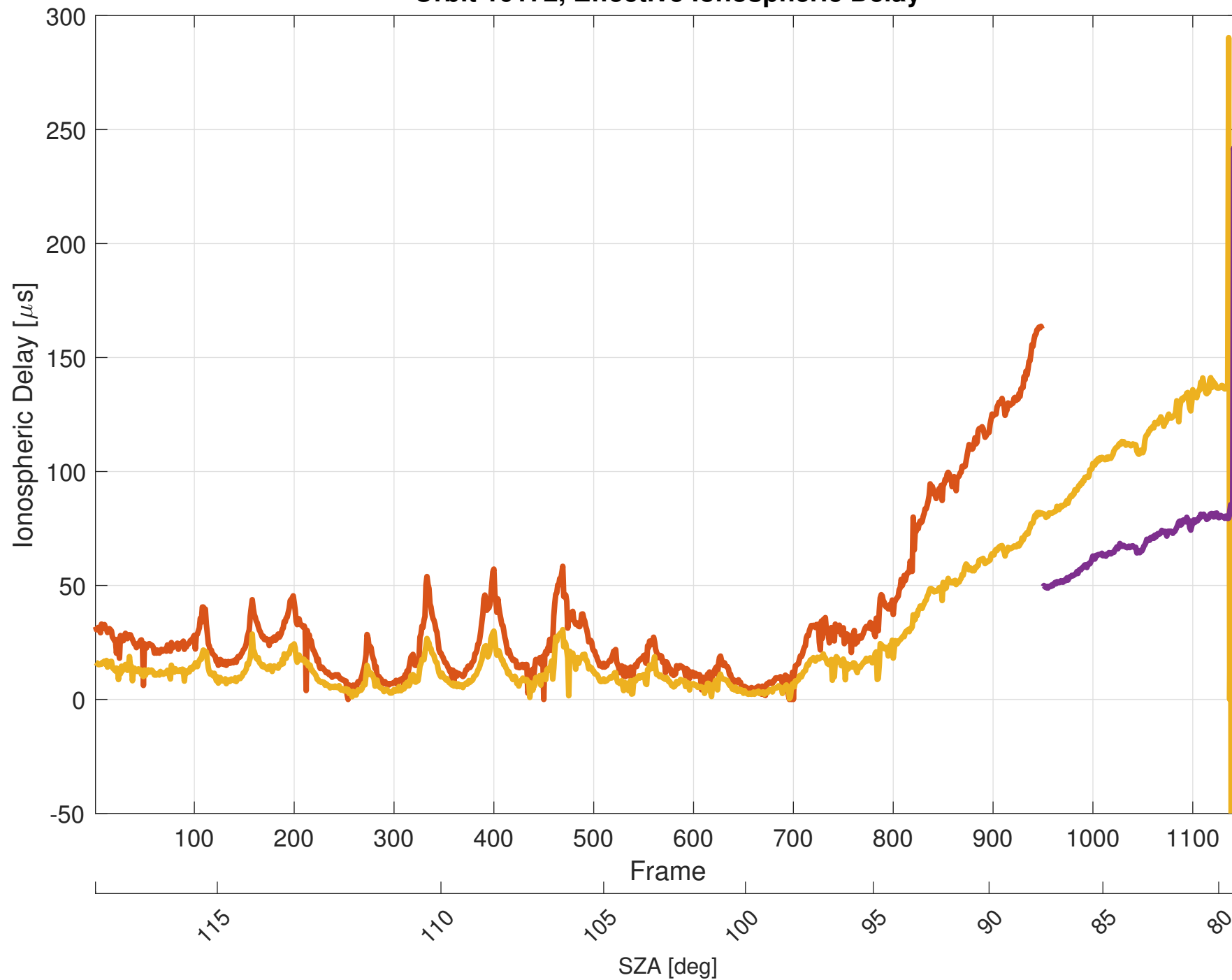
Orbit 10172, Effective Ionospheric Delay
