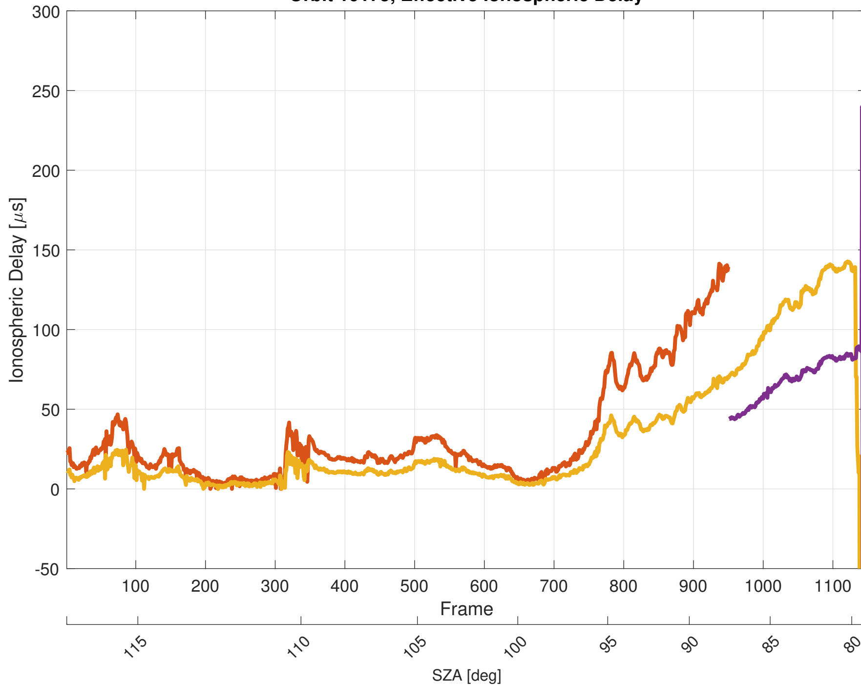
Orbit 10175, Effective Ionospheric Delay
