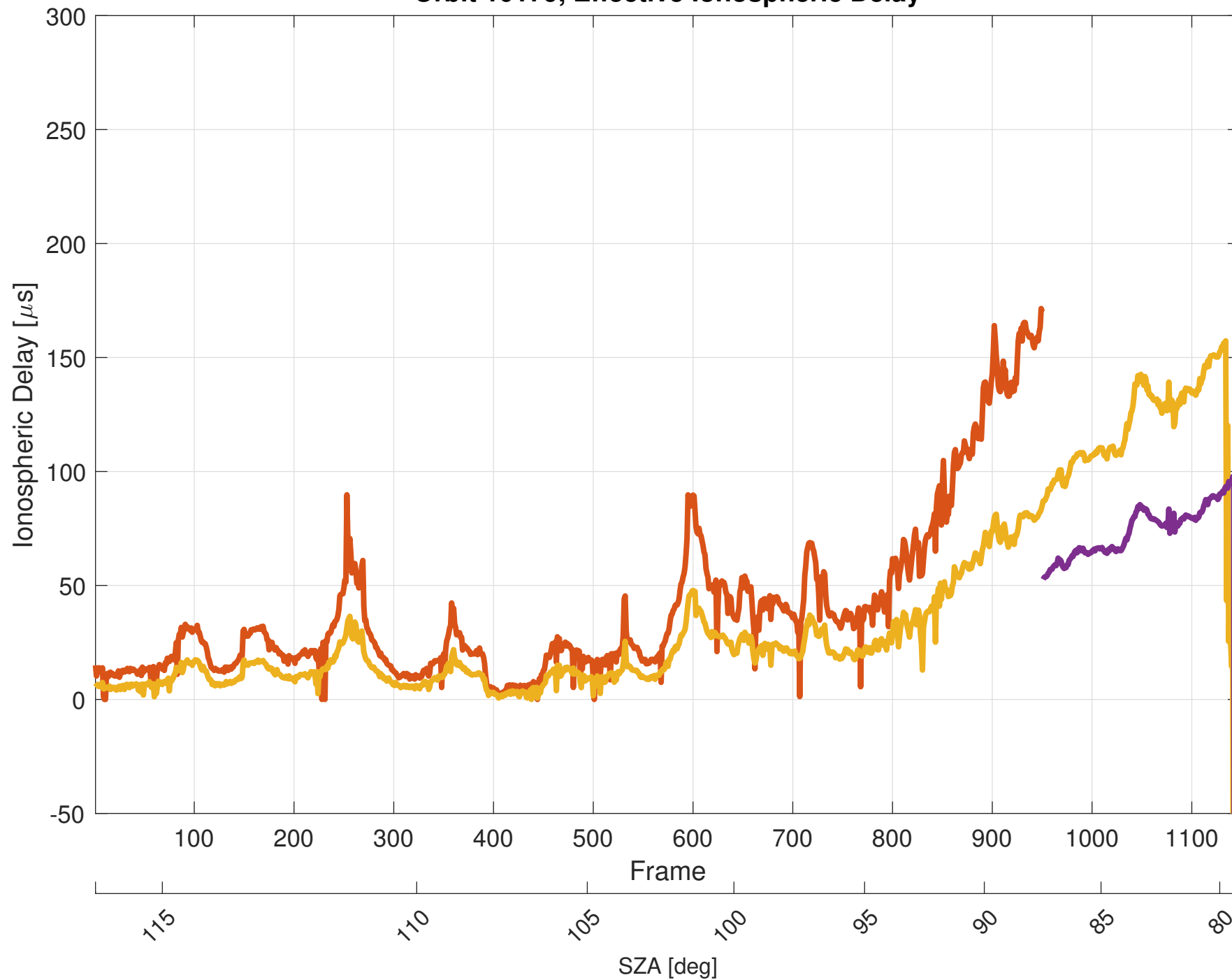
Orbit 10179, Effective Ionospheric Delay
