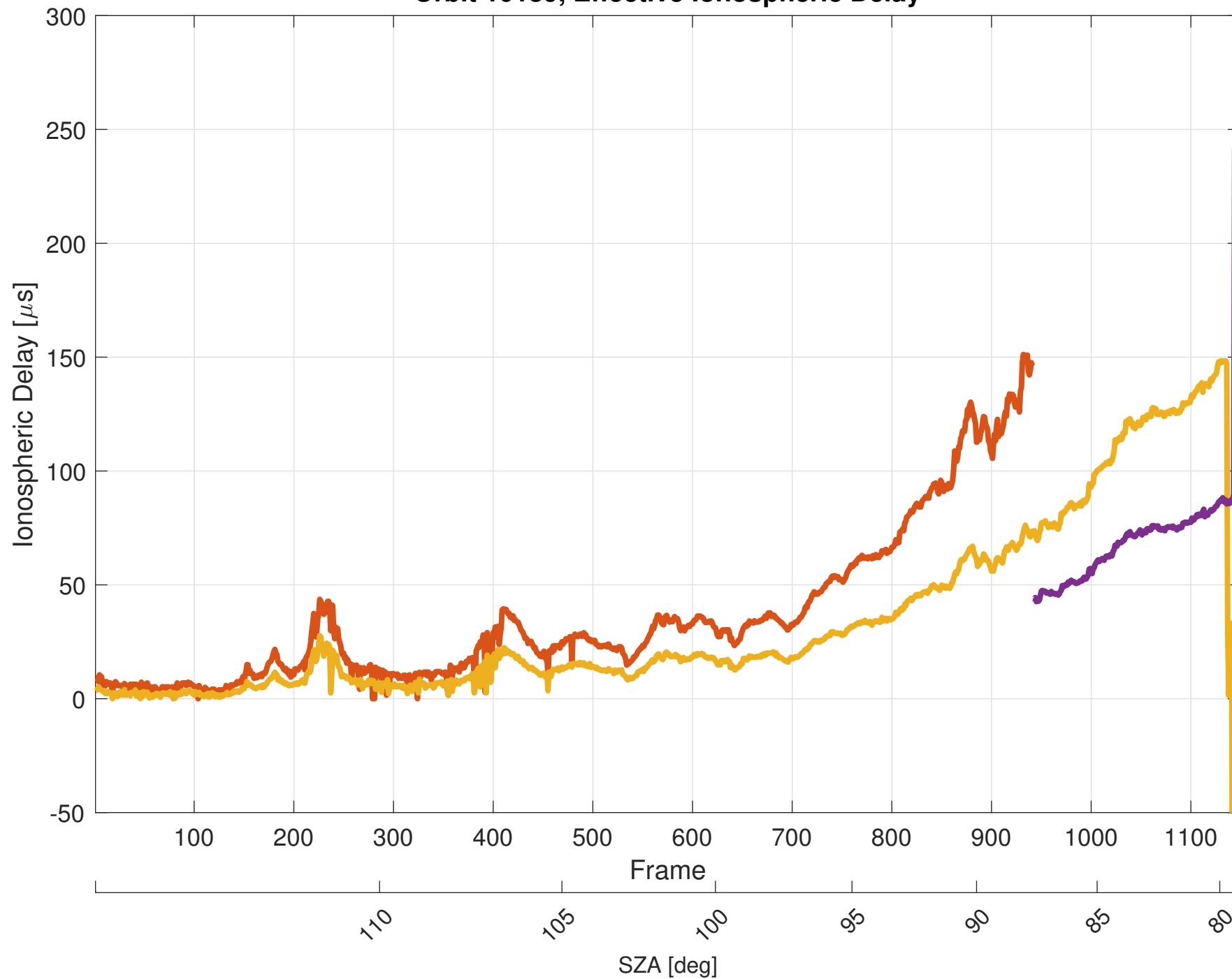
Orbit 10189, Effective Ionospheric Delay
