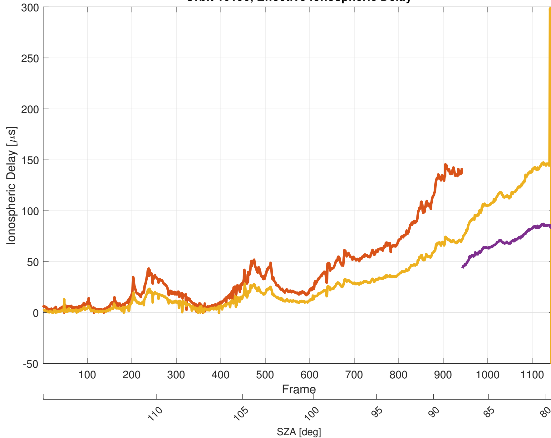
Orbit 10196, Effective Ionospheric Delay
