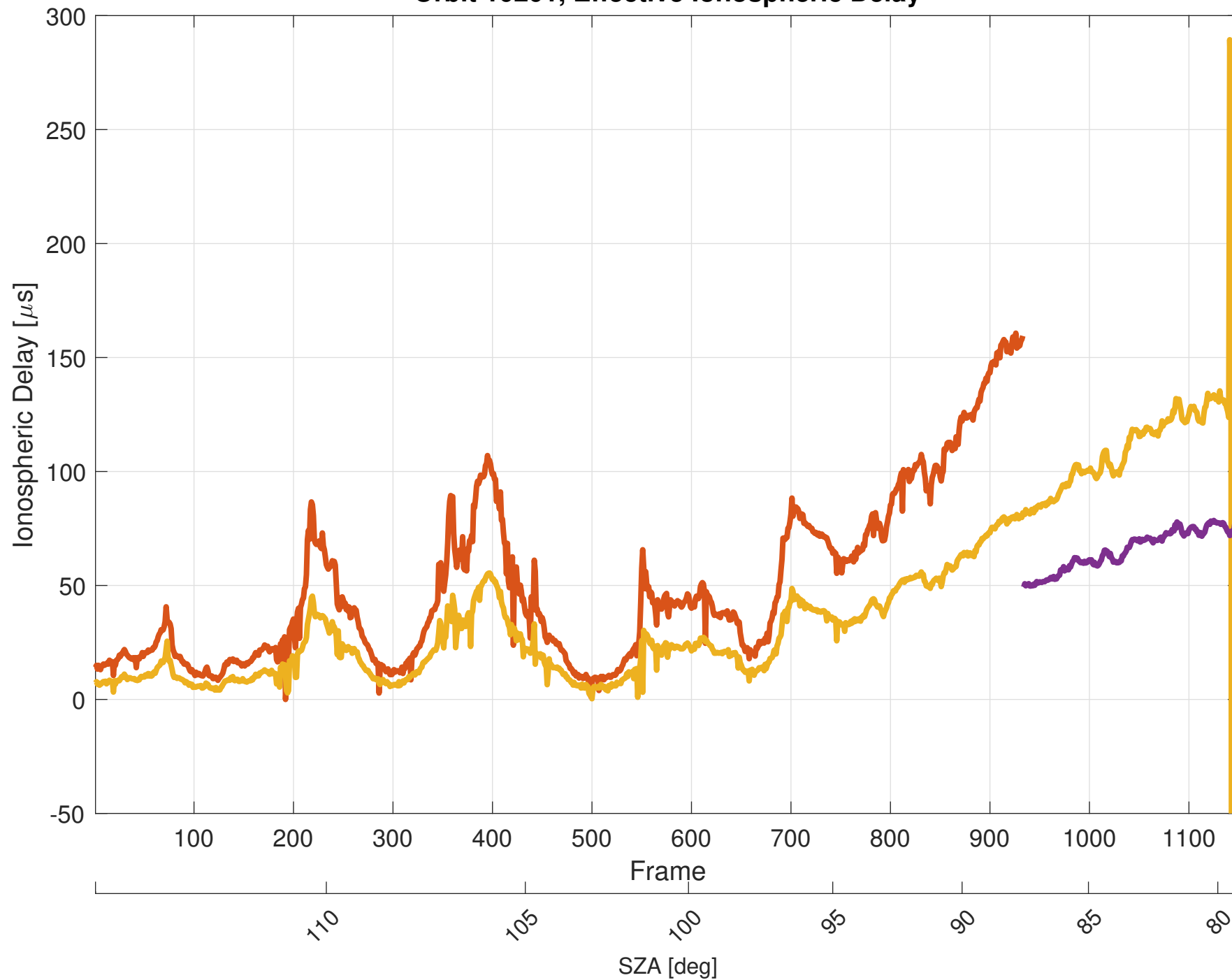
Orbit 10201, Effective Ionospheric Delay
