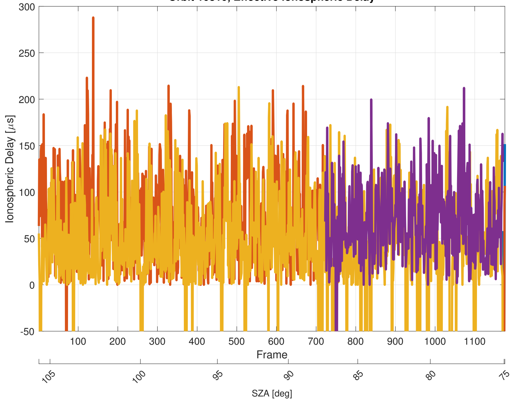
Orbit 10310, Effective Ionospheric Delay
