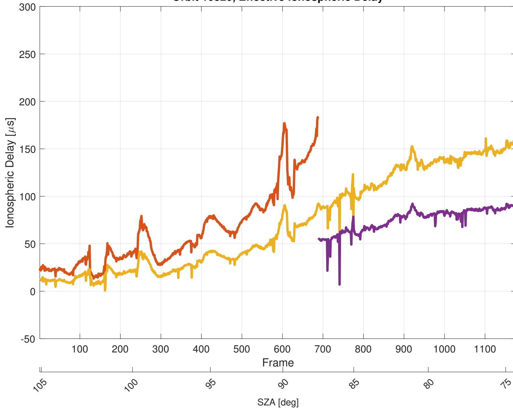
Orbit 10320, Effective Ionospheric Delay
