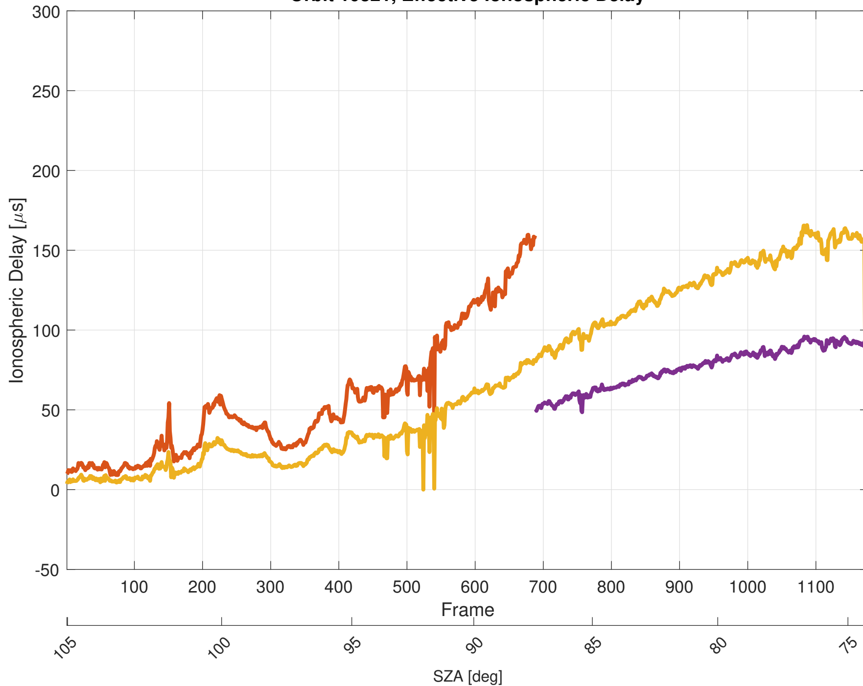
Orbit 10321, Effective Ionospheric Delay
