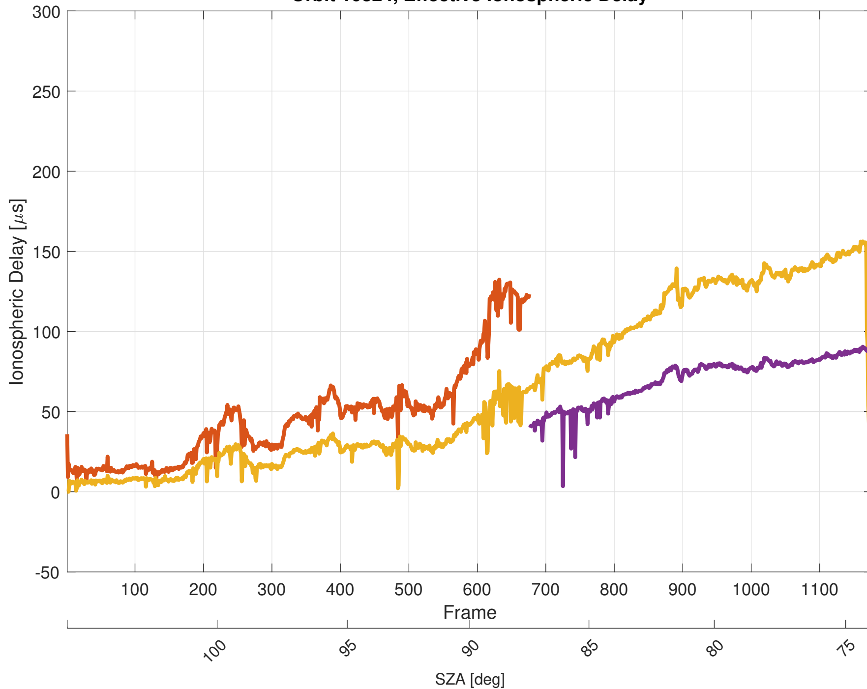
Orbit 10324, Effective Ionospheric Delay
