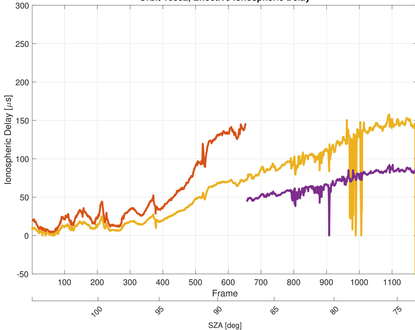
Orbit 10332, Effective Ionospheric Delay
