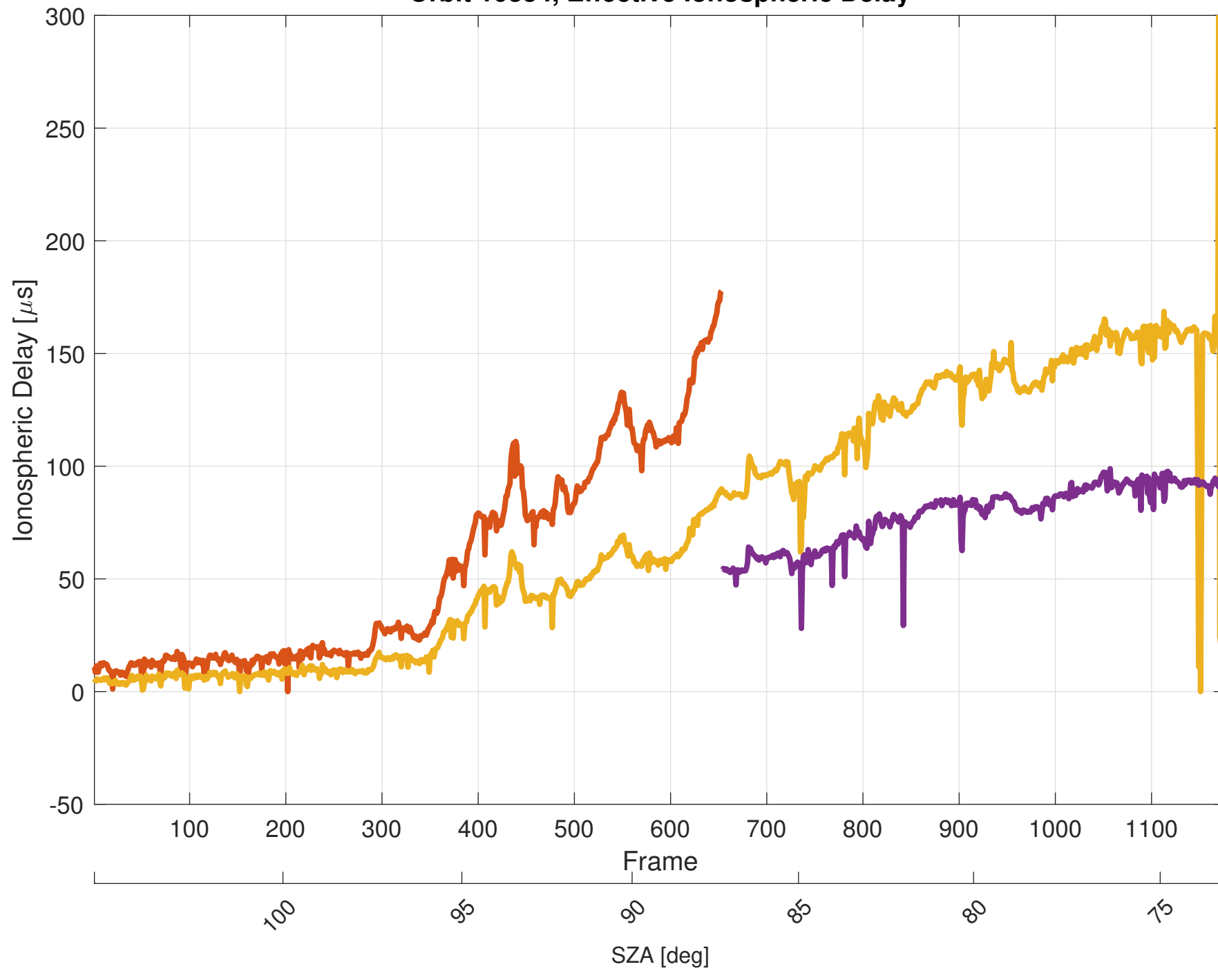
Orbit 10334, Effective Ionospheric Delay
