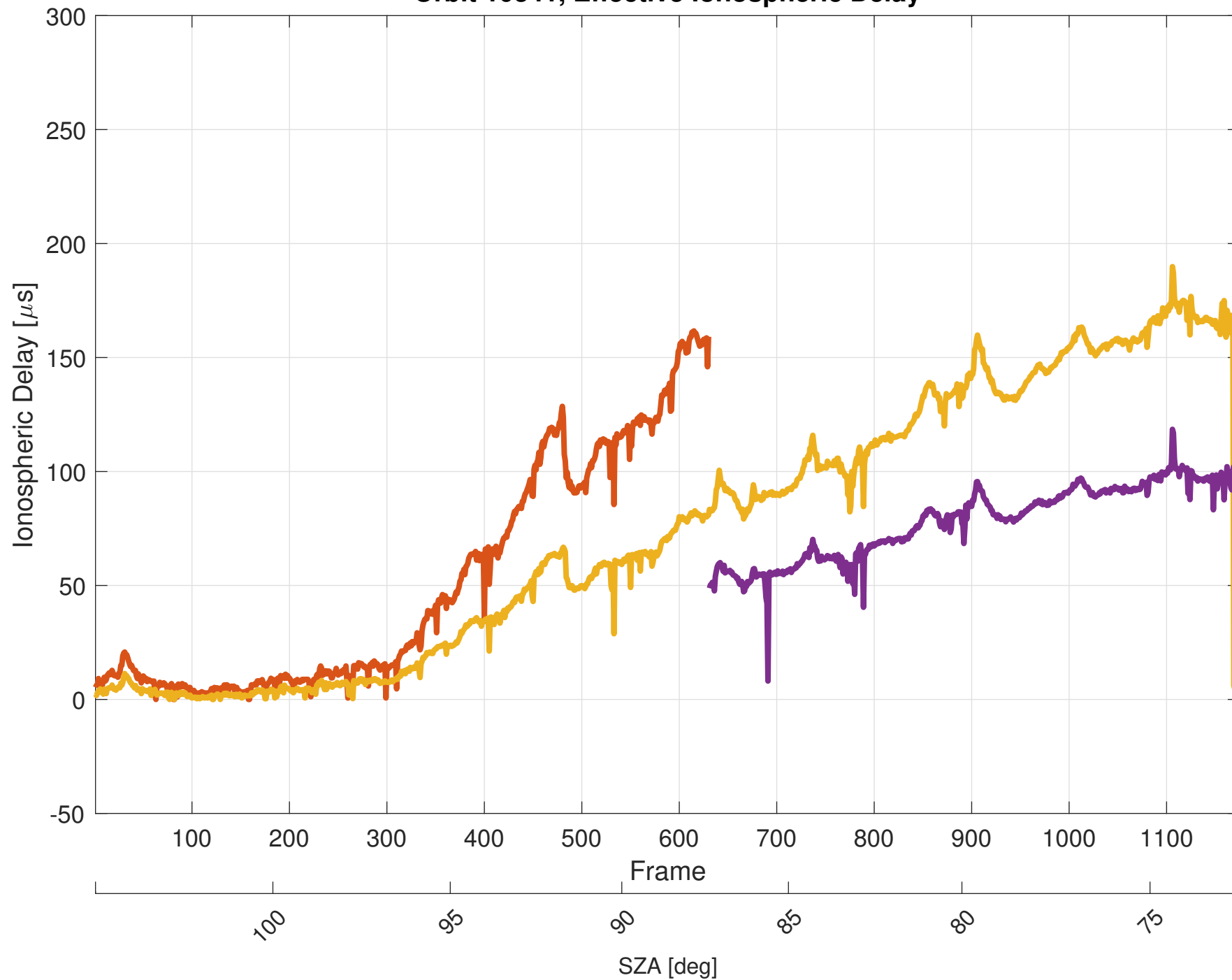
Orbit 10341, Effective Ionospheric Delay
