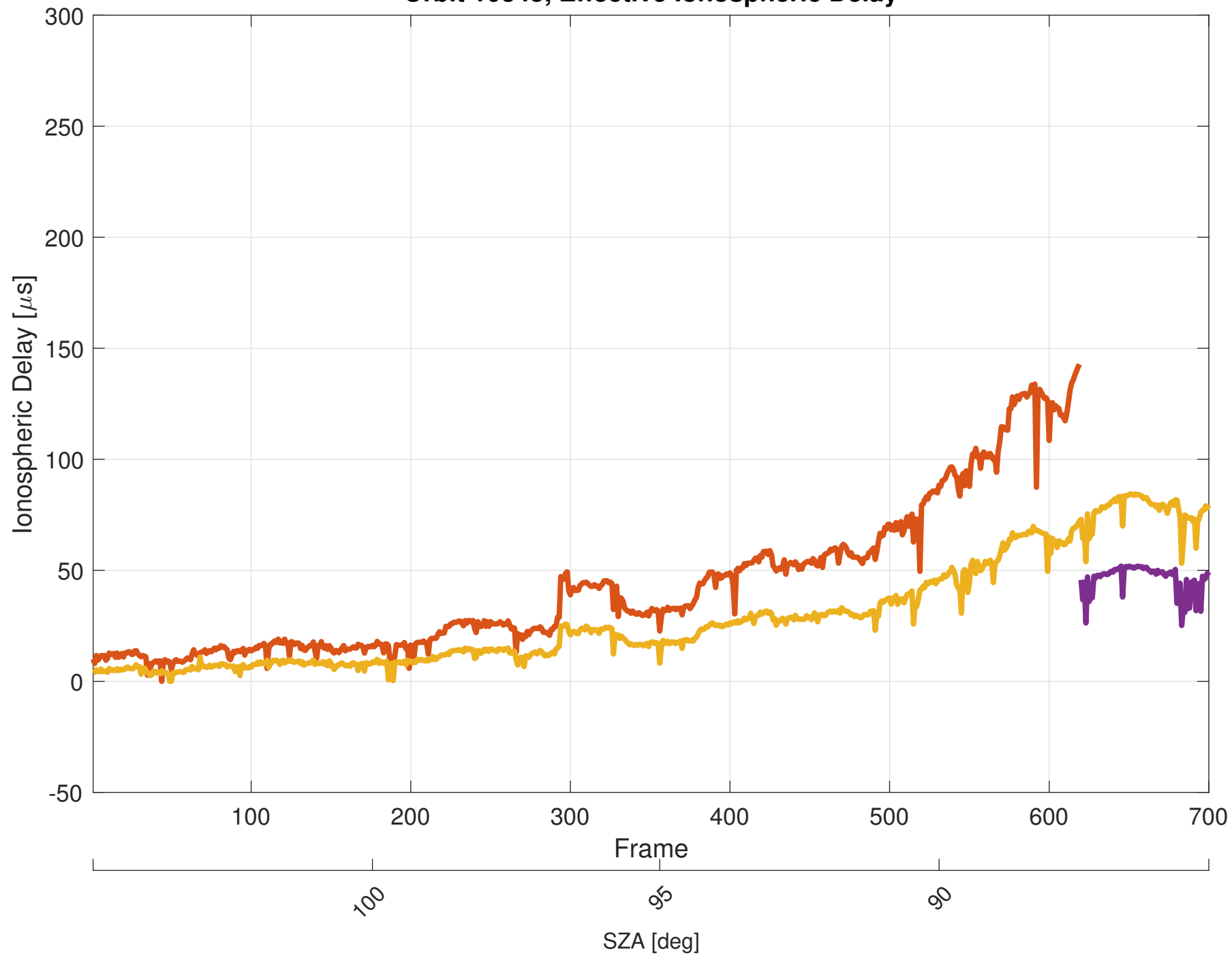
Orbit 10345, Effective Ionospheric Delay
