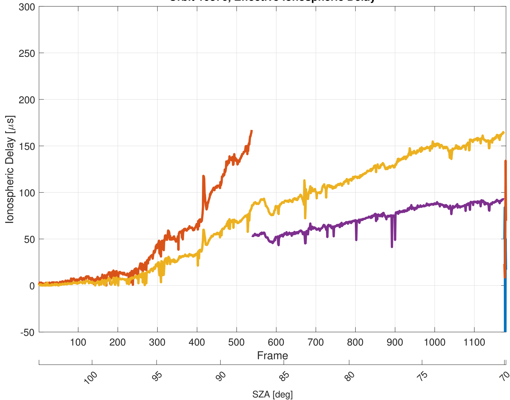
Orbit 10376, Effective Ionospheric Delay
