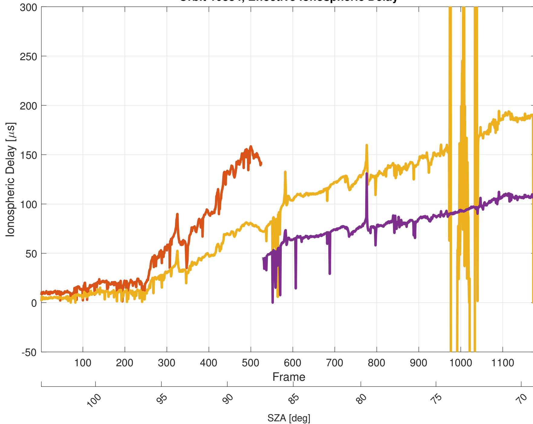
Orbit 10384, Effective Ionospheric Delay
