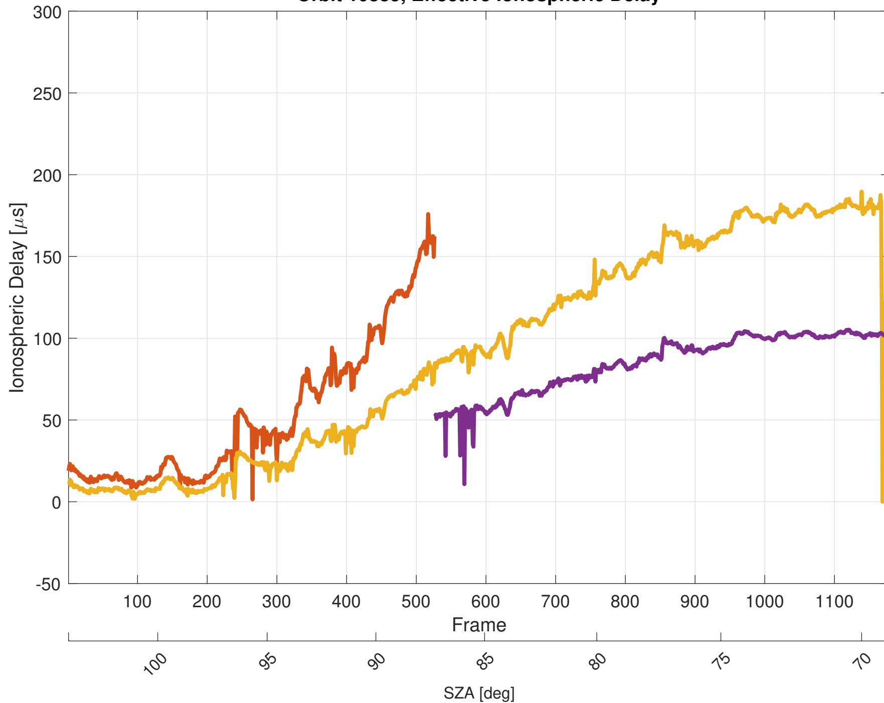
Orbit 10385, Effective Ionospheric Delay
