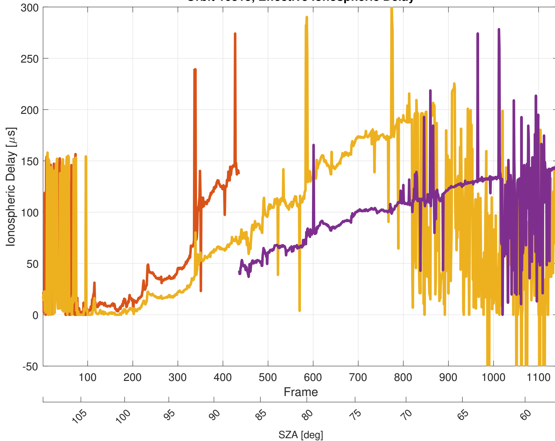
Orbit 10515, Effective Ionospheric Delay
