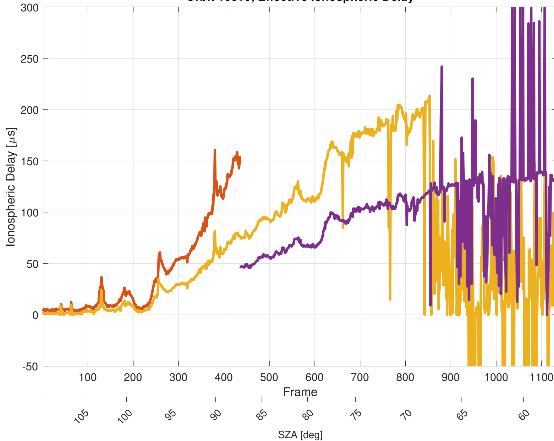
Orbit 10519, Effective Ionospheric Delay
