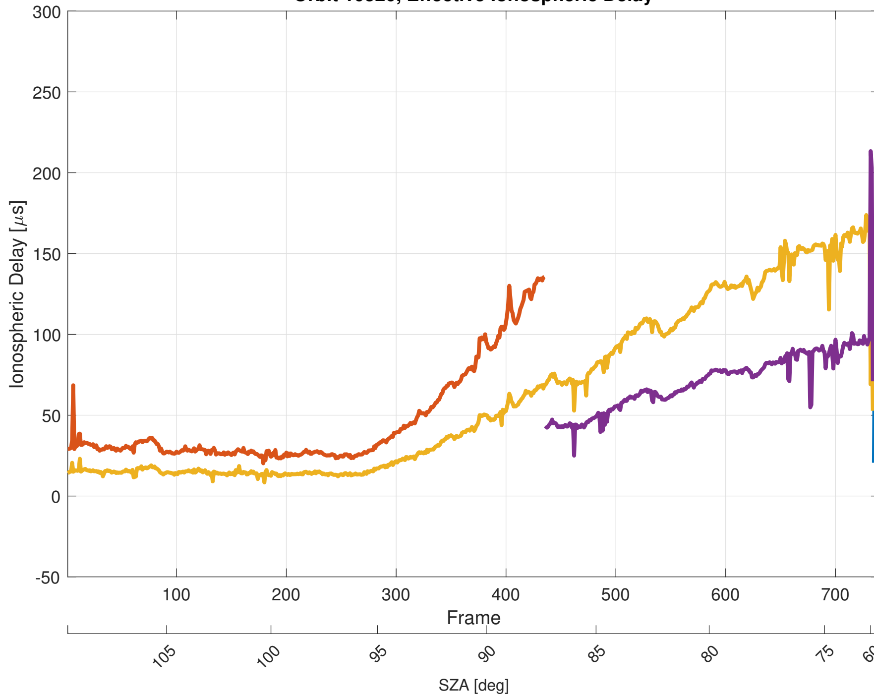
Orbit 10520, Effective Ionospheric Delay
