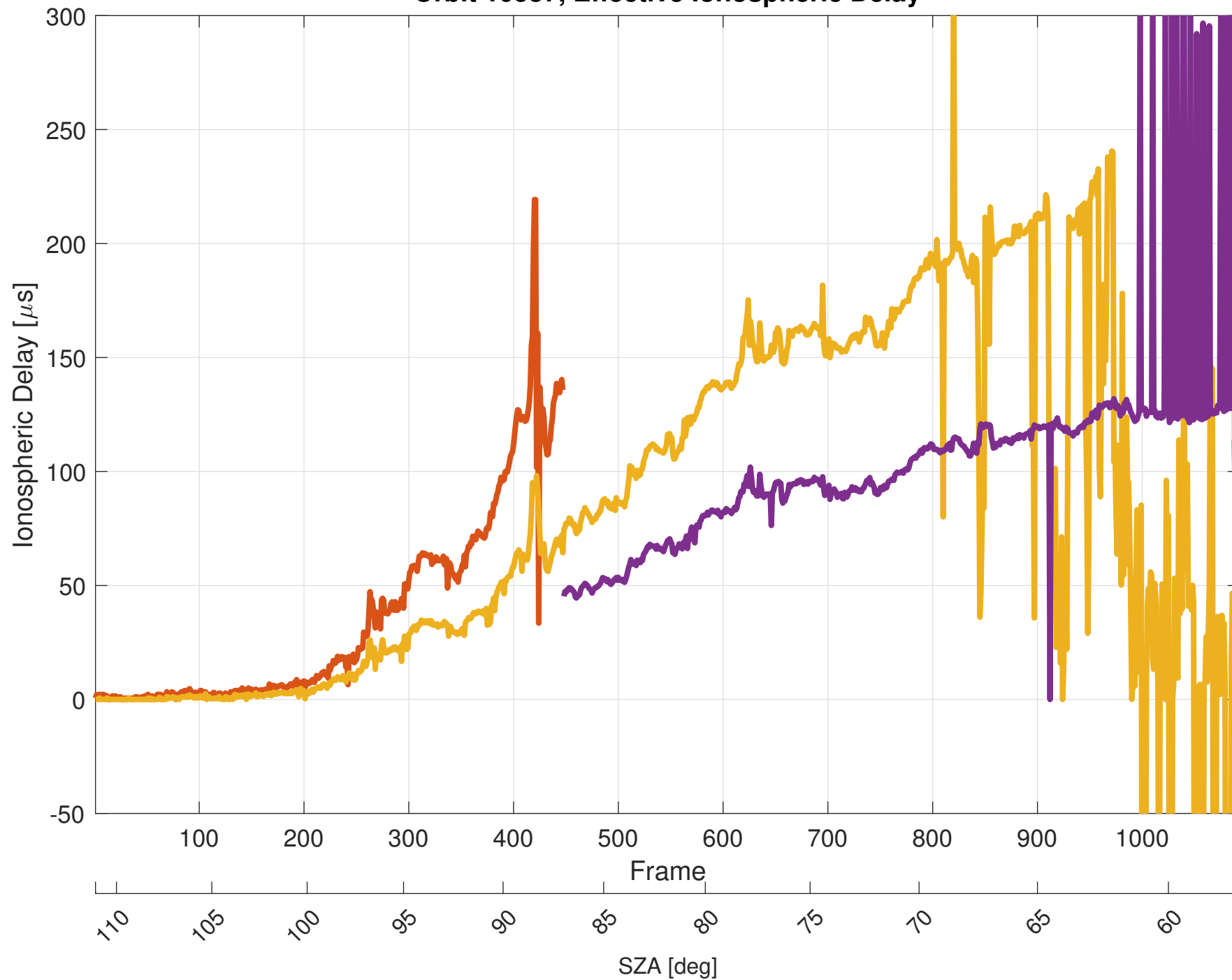
Orbit 10537, Effective Ionospheric Delay
